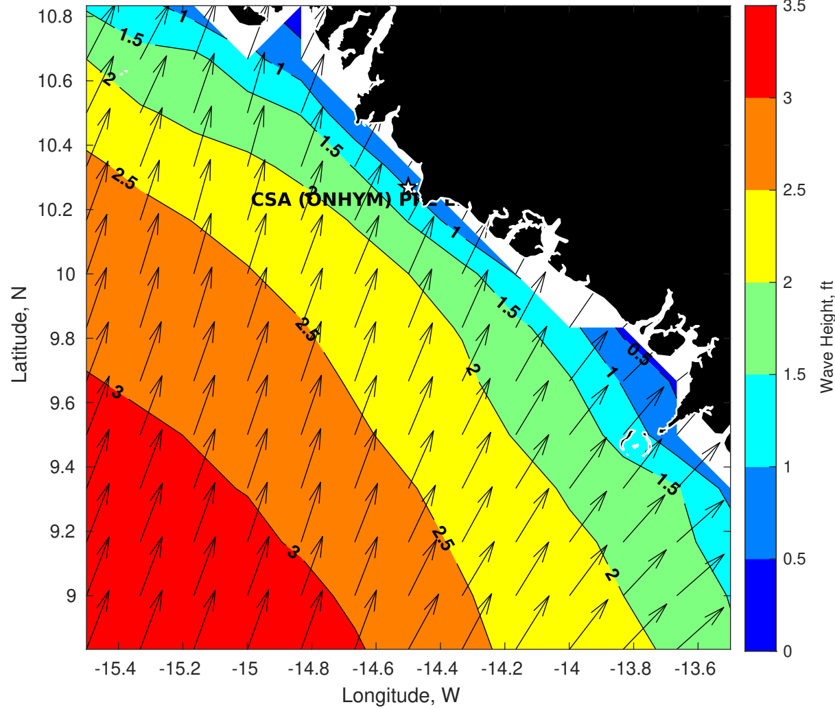
Wave Height (ft) for CSA (ONHYM) PPL EBS - Guinea at 07-Jun-2025 09:00:00
