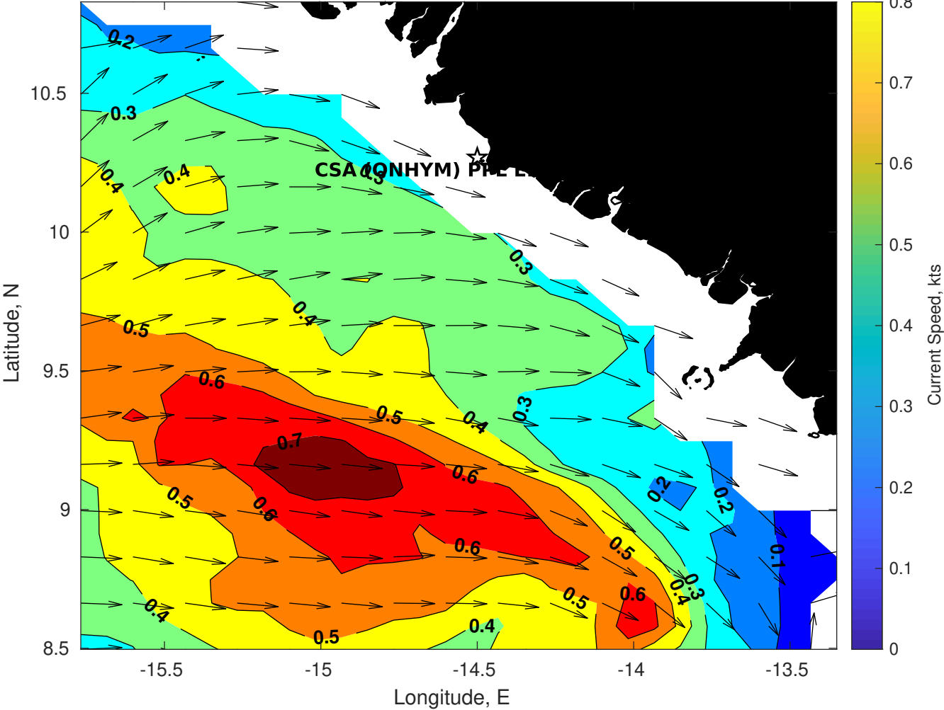
Surface Currents for CSA (ONHYM) PPL EBS - Guinea at 06-Jun-2025 00:00:00
