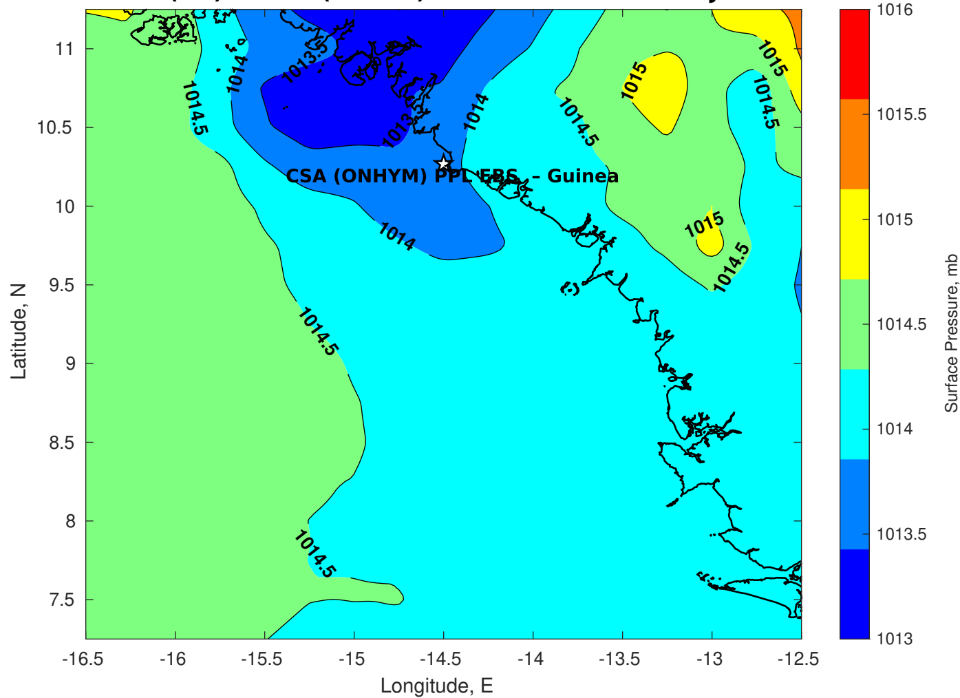
Surface Pressure (mb) for CSA (ONHYM) PPL EBS - Guinea at 08-Jun-2025 00:00:00
