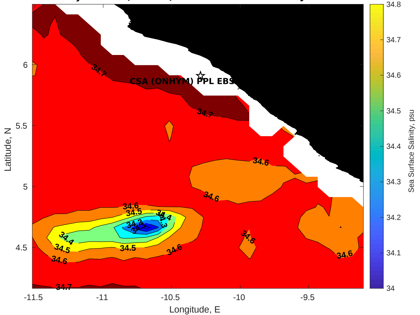
Surface Salinity for CSA (ONHYM) PPL EBS - Liberia at 06-Jun-2025 00:00:00
