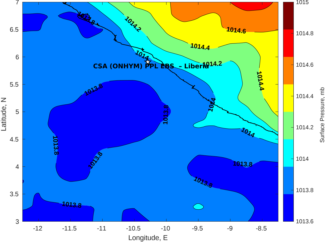
Surface Pressure (mb) for CSA (ONHYM) PPL EBS - Liberia at 09-Jun-2025 00:00:00
