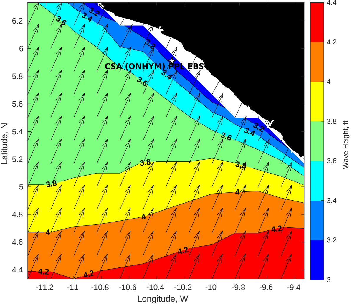
Wave Height (ft) for CSA (ONHYM) PPL EBS - Liberia at 07-Jun-2025 09:00:00
