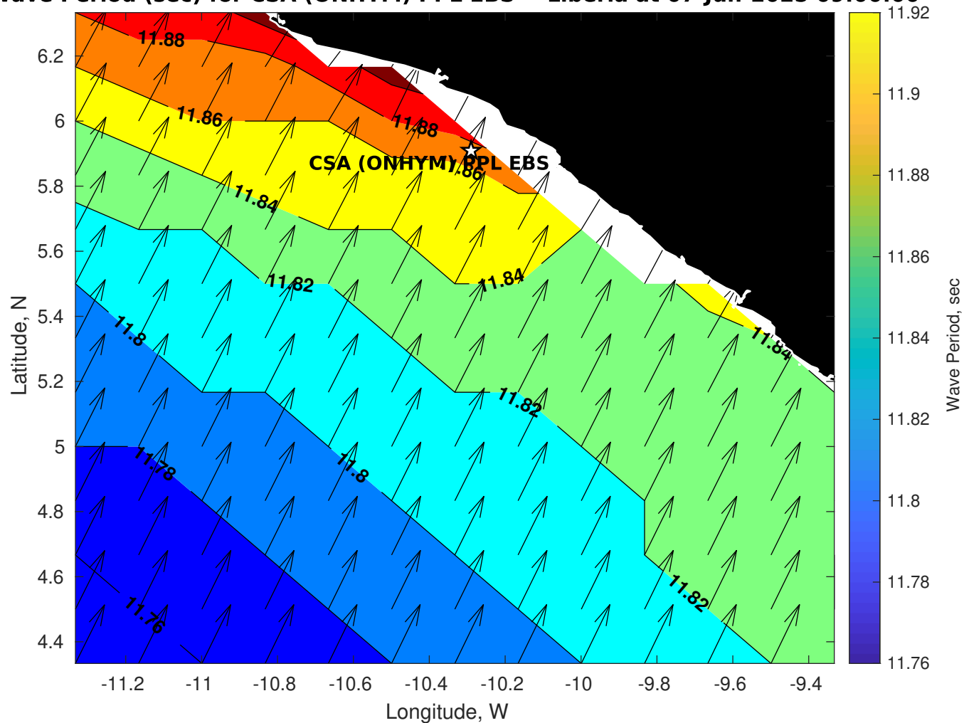
Wave Period (sec) for CSA (ONHYM) PPL EBS - Liberia at 07-Jun-2025 09:00:00
