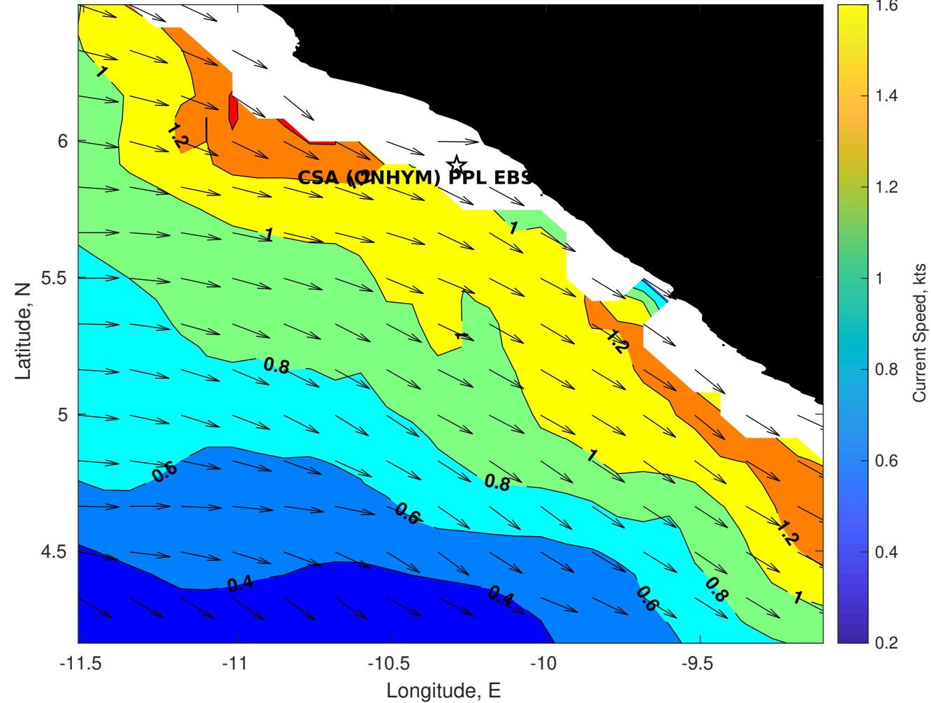
Surface Currents for CSA (ONHYM) PPL EBS - Liberia at 06-Jun-2025 00:00:00
