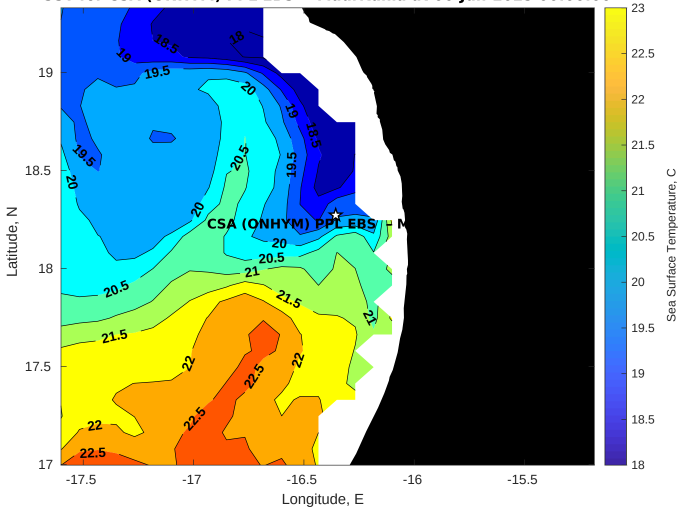
SST for CSA (ONHYM) PPL EBS - Mauritania at 06-Jun-2025 00:00:00
