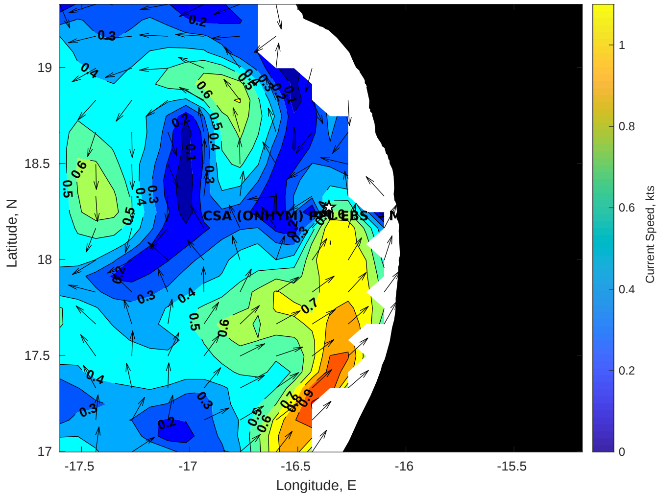
Surface Currents for CSA (ONHYM) PPL EBS - Mauritania at 06-Jun-2025 00:00:00
