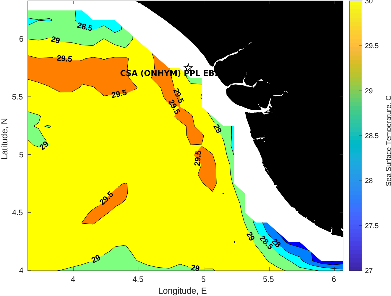
SST for CSA (ONHYM) PPL EBS - Nigeria at 06-Jun-2025 00:00:00
