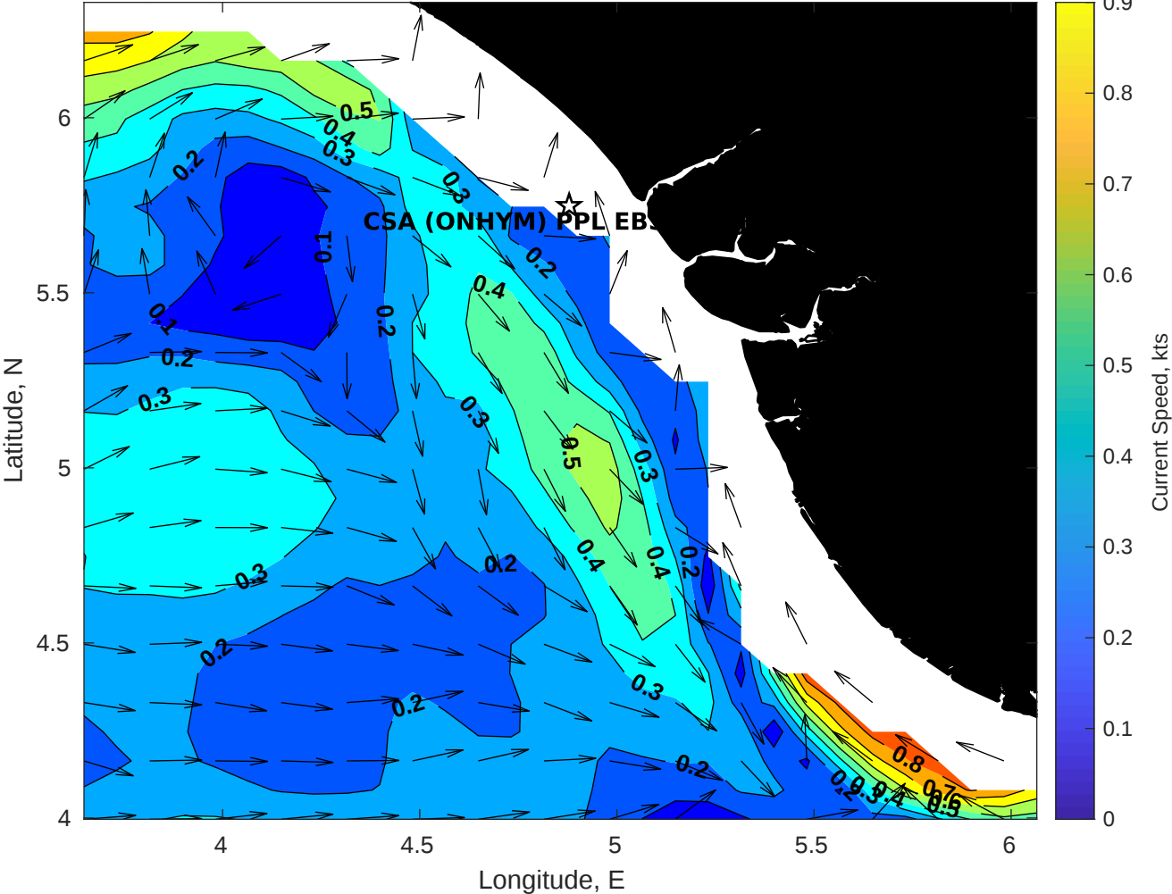
Surface Currents for CSA (ONHYM) PPL EBS - Nigeria at 06-Jun-2025 00:00:00
