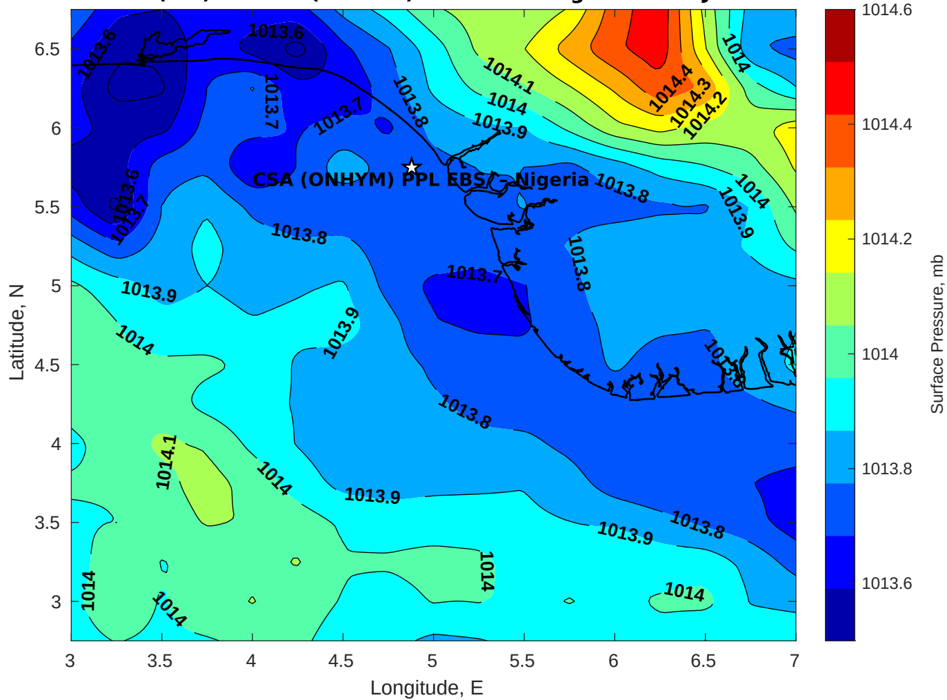
Surface Pressure (mb) for CSA (ONHYM) PPL EBS - Nigeria at 07-Jun-2025 00:00:00
