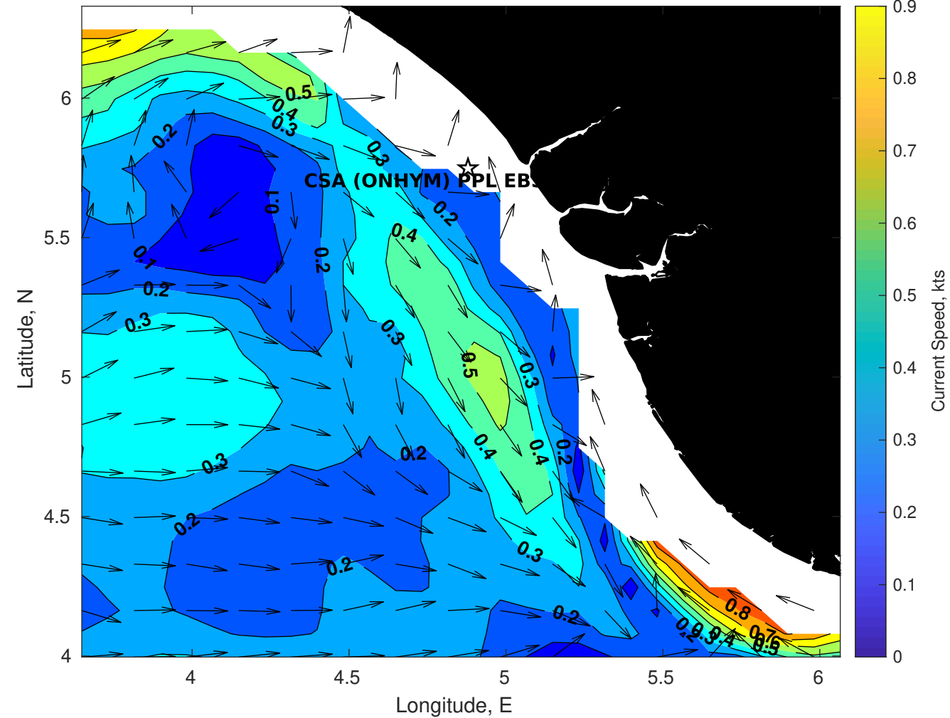
Surface Currents for CSA (ONHYM) PPL EBS - Nigeria at 06-Jun-2025 00:00:00
