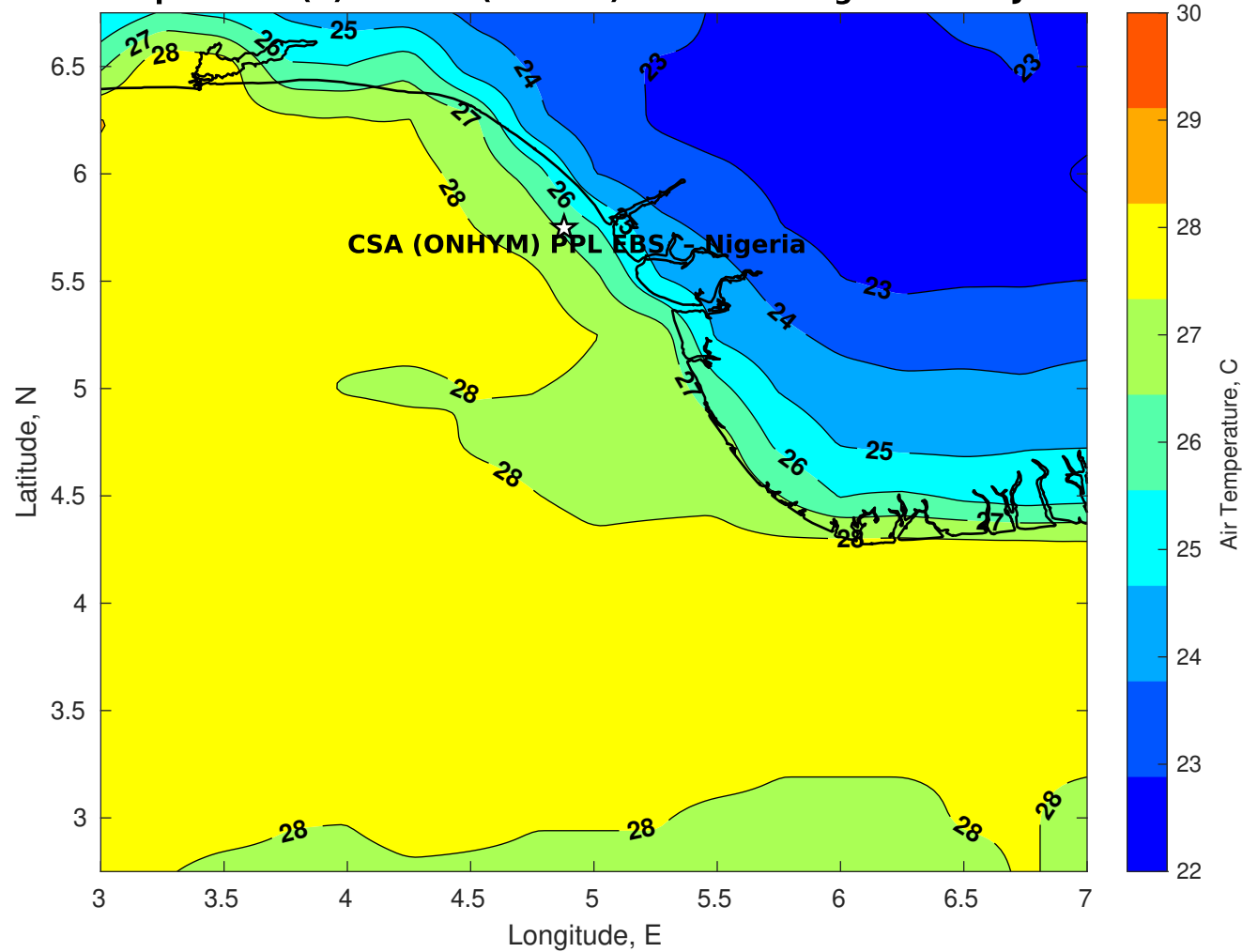
Air Temperature (C) for CSA (ONHYM) PPL EBS - Nigeria at 07-Jun-2025
