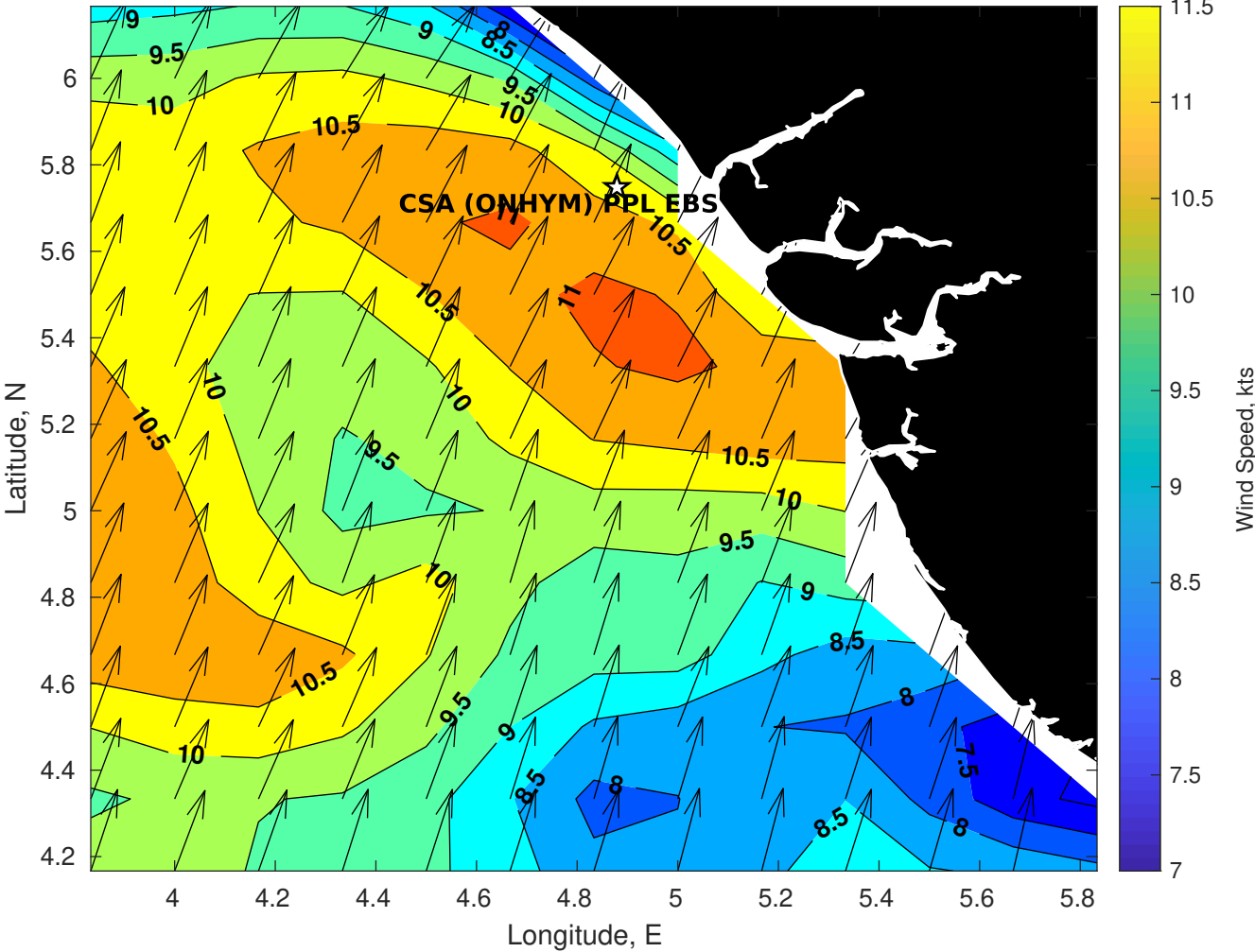
Winds (kts) for CSA (ONHYM) PPL EBS - Nigeria at 07-Jun-2025 09:00:00
