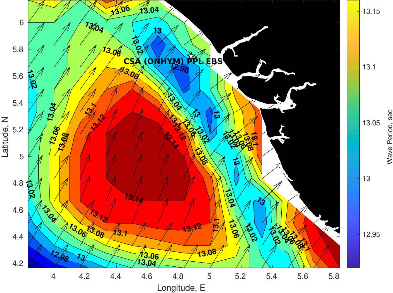
Wave Period (sec) for CSA (ONHYM) PPL EBS - Nigeria at 07-Jun-2025 09:00:00
