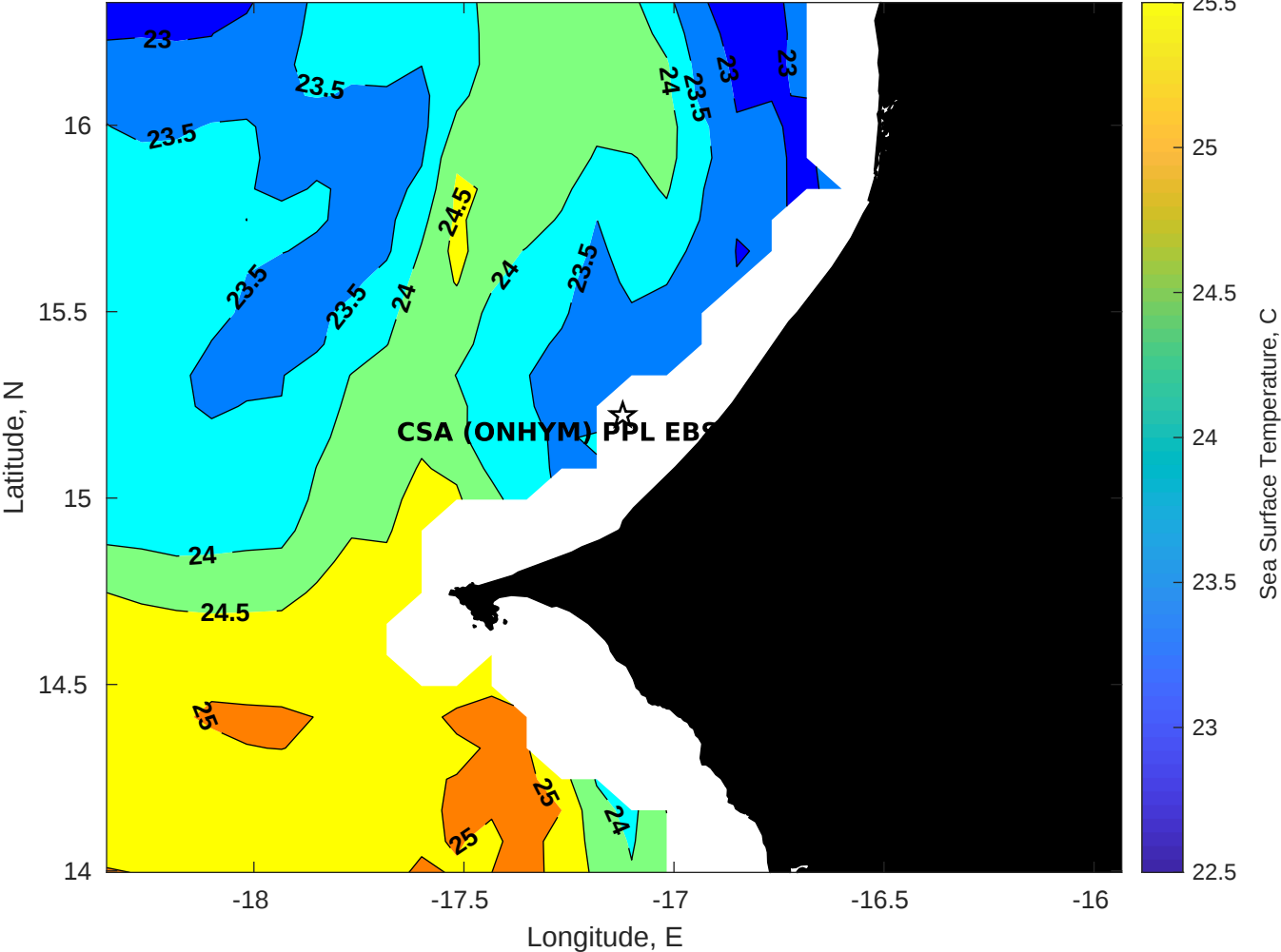
SST for CSA (ONHYM) PPL EBS - Senegal at 06-Jun-2025 00:00:00
