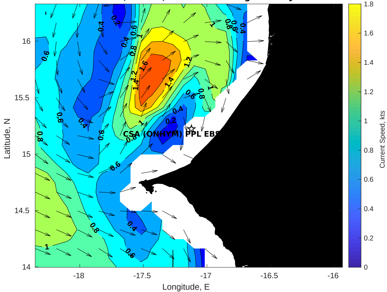
Surface Currents for CSA (ONHYM) PPL EBS - Senegal at 06-Jun-2025 00:00:00
