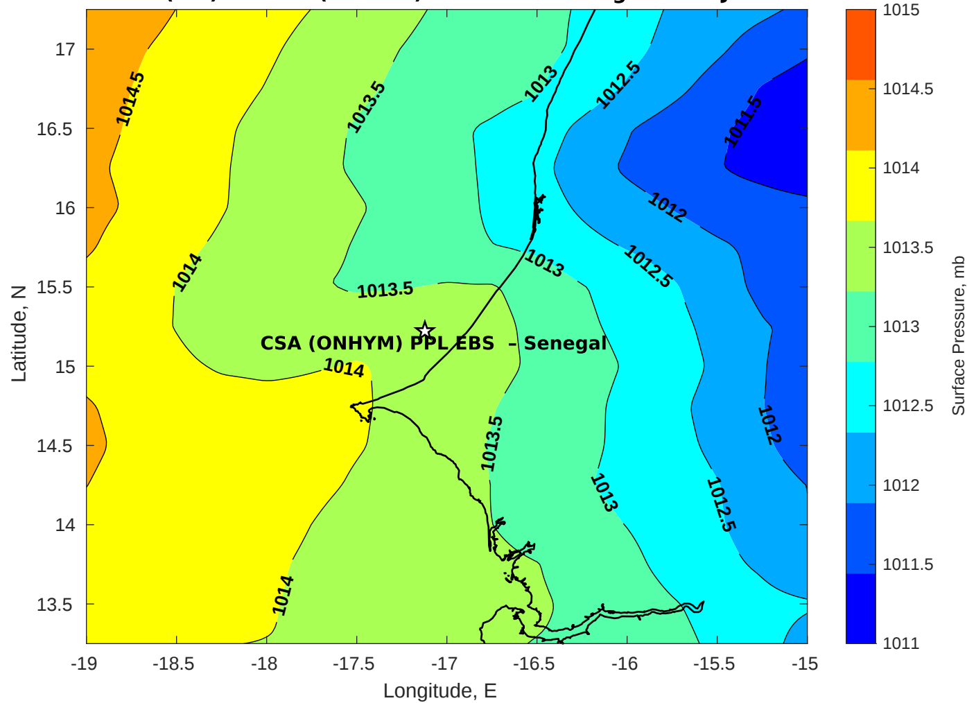
Surface Pressure (mb) for CSA (ONHYM) PPL EBS - Senegal at 07-Jun-2025 00:00:00
