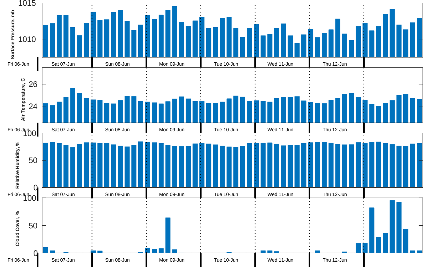
Met Forecast for CSA (ONHYM) PPL EBS - Senegal from 07-Jun-2025 00:00:00 to 14-Jun-2025 00:00:00
