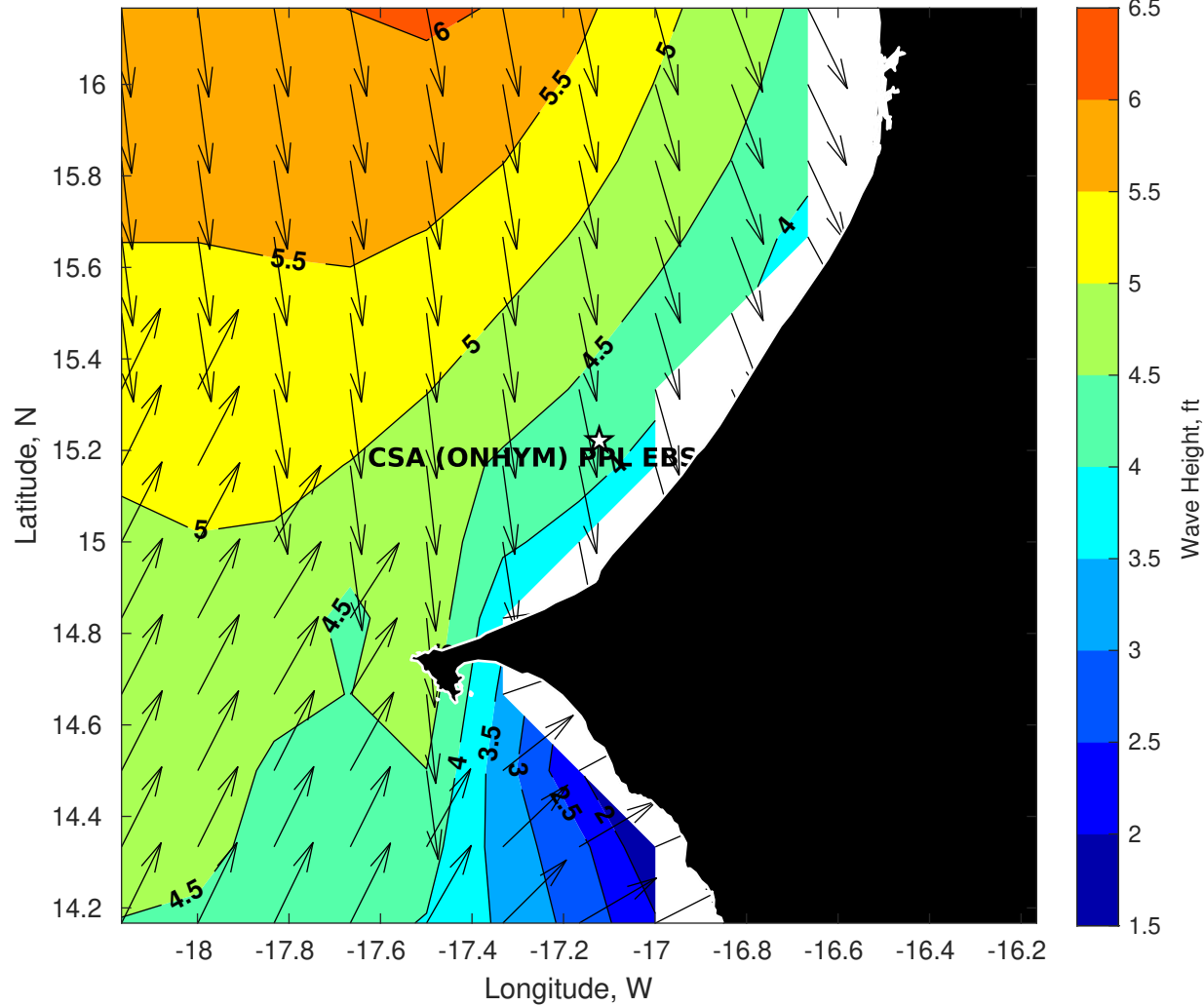
Wave Height (ft) for CSA (ONHYM) PPL EBS - Senegal at 07-Jun-2025 09:00:00
