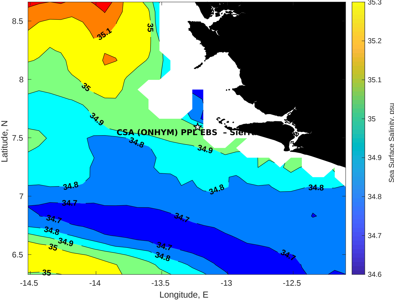
Surface Salinity for CSA (ONHYM) PPL EBS - Sierra Leone at 06-Jun-2025 00:00:00
