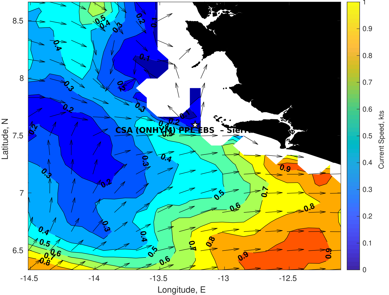
Surface Currents for CSA (ONHYM) PPL EBS - Sierra Leone at 06-Jun-2025 00:00:00
