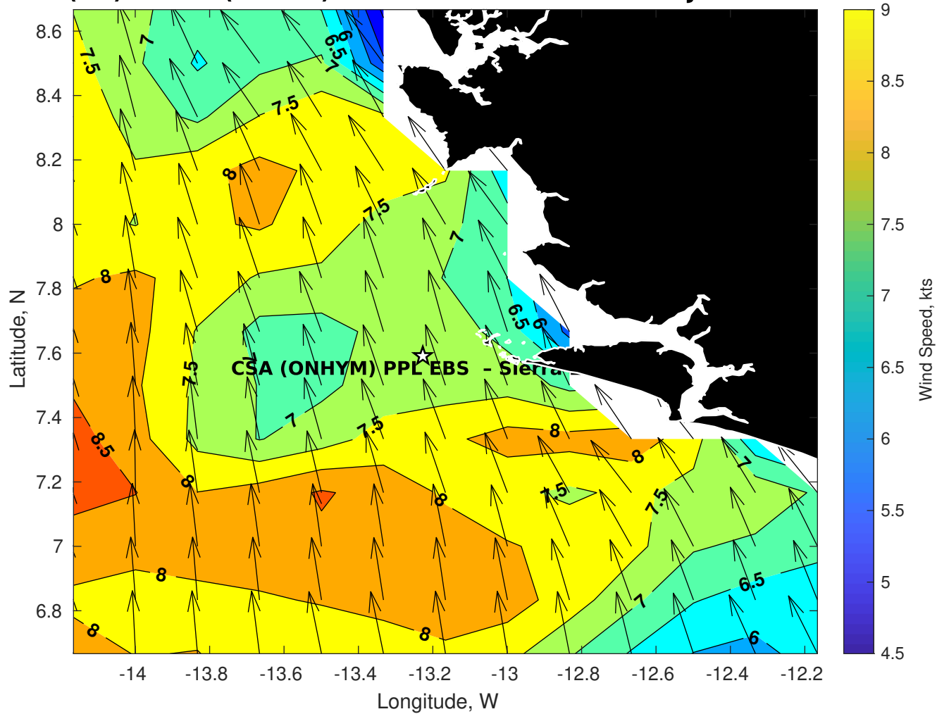
Winds (kts) for CSA (ONHYM) PPL EBS - Sierra Leone at 07-Jun-2025 09:00:00
