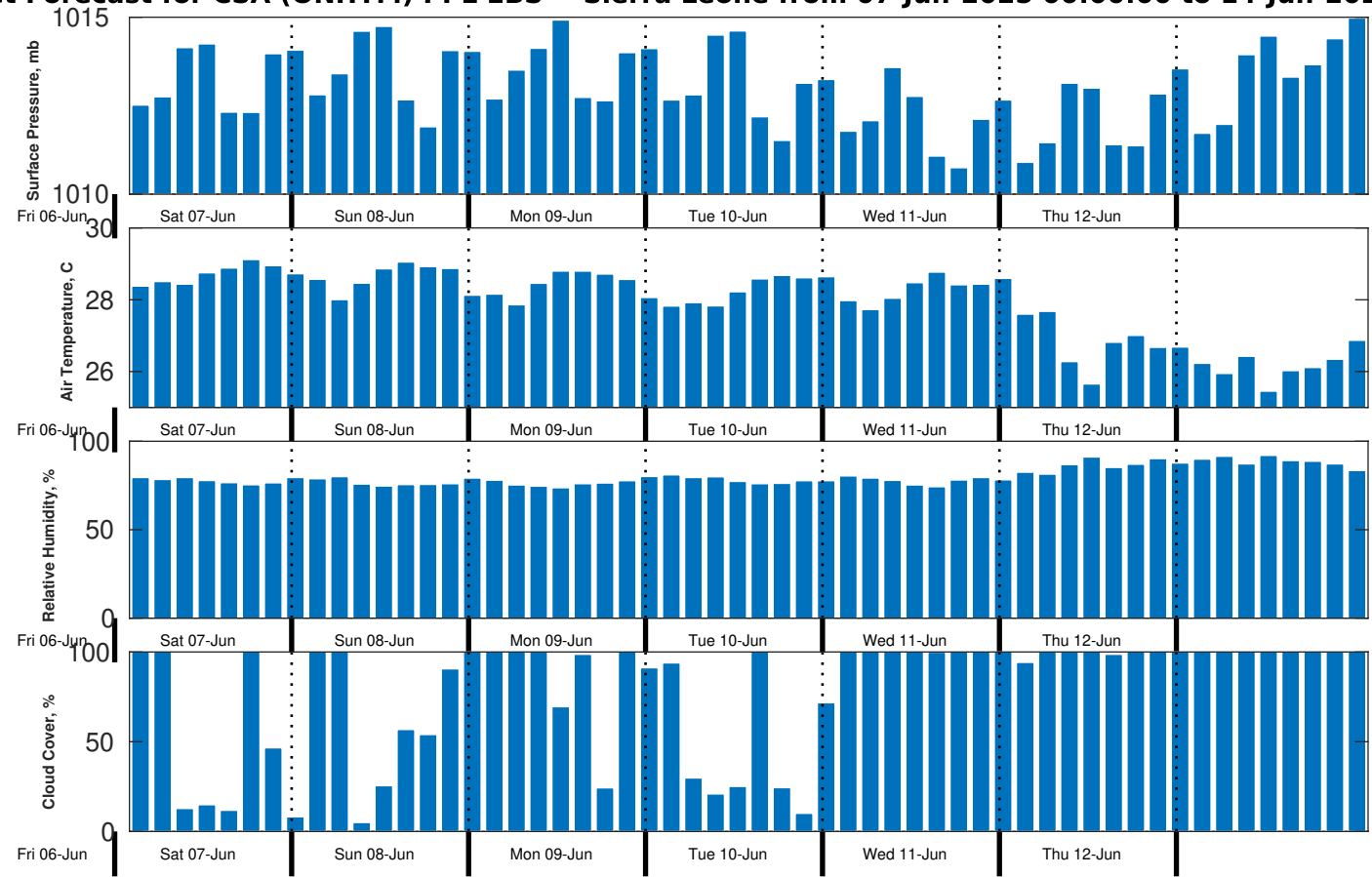
Met Forecast for CSA (ONHYM) PPL EBS - Sierra Leone from 07-Jun-2025 00:00:00 to 14-Jun-2025 00:00:00
