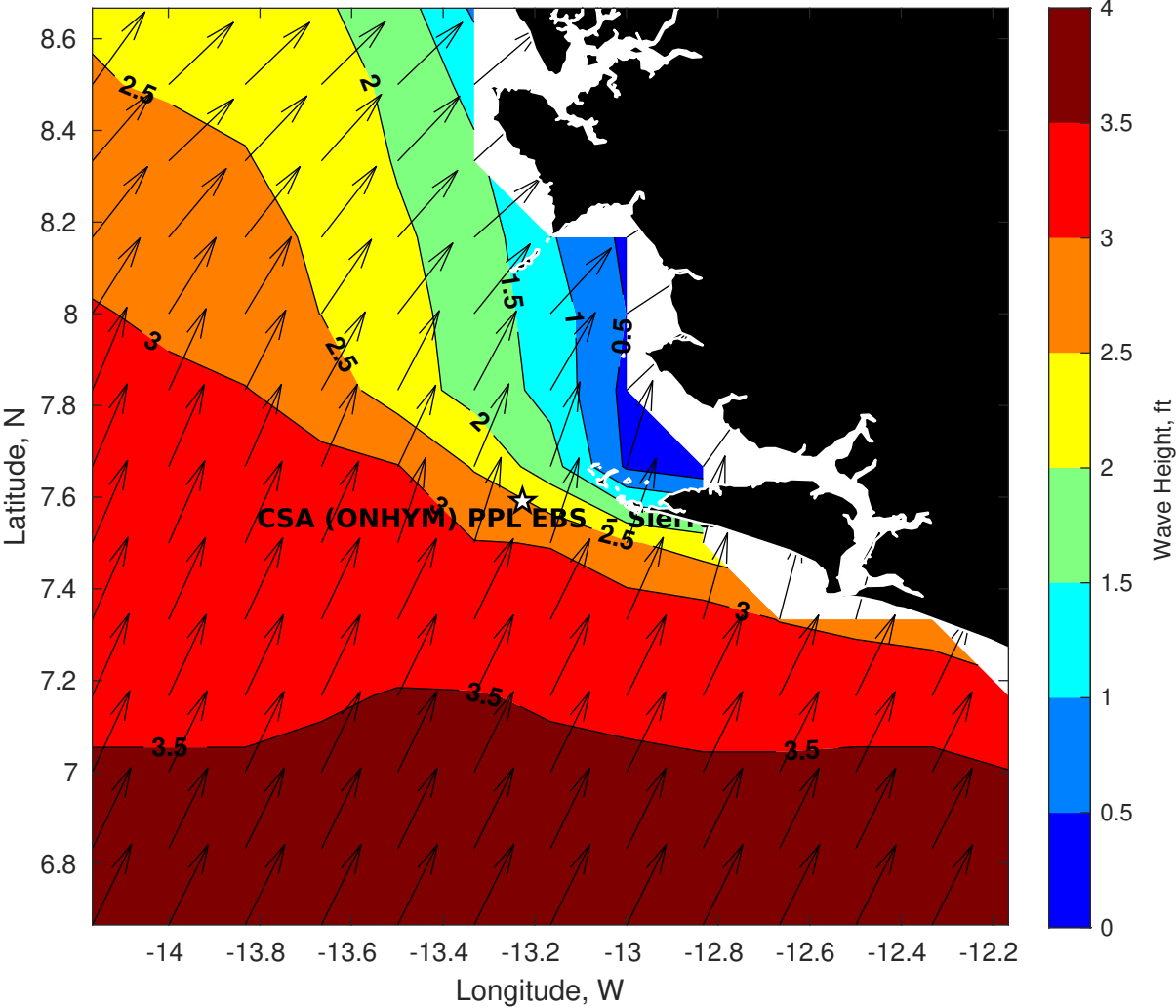
Wave Height (ft) for CSA (ONHYM) PPL EBS - Sierra Leone at 07-Jun-2025 09:00:00
