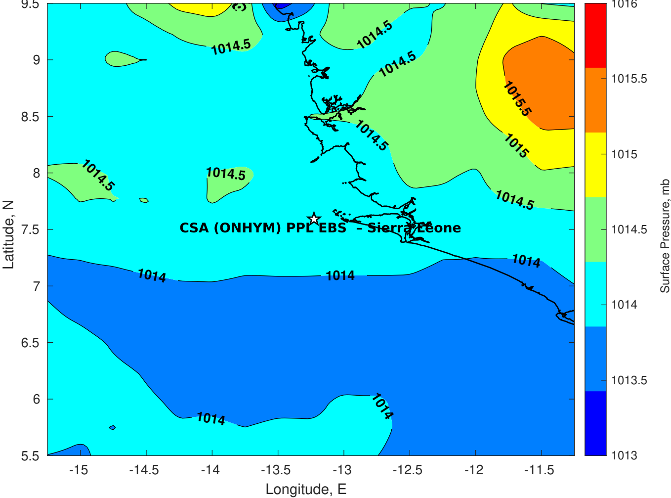
Surface Pressure (mb) for CSA (ONHYM) PPL EBS - Sierra Leone at 09-Jun-2025 00:00:00
