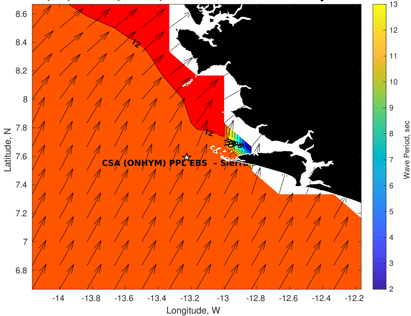
Wave Period (sec) for CSA (ONHYM) PPL EBS - Sierra Leone at 07-Jun-2025 09:00:00
