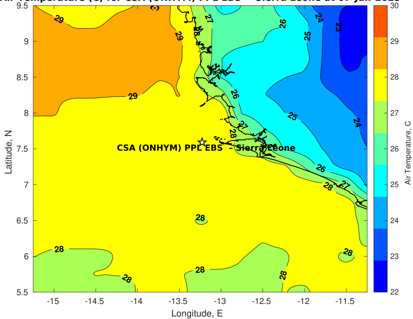
Air Temperature (C) for CSA (ONHYM) PPL EBS - Sierra Leone at 07-Jun-2025
