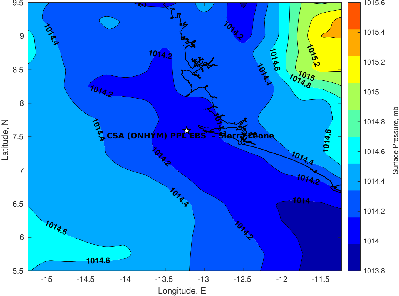
Surface Pressure (mb) for CSA (ONHYM) PPL EBS - Sierra Leone at 08-Jun-2025 00:00:00
