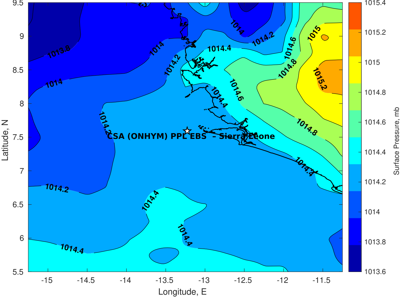
Surface Pressure (mb) for CSA (ONHYM) PPL EBS - Sierra Leone at 07-Jun-2025 00:00:00
