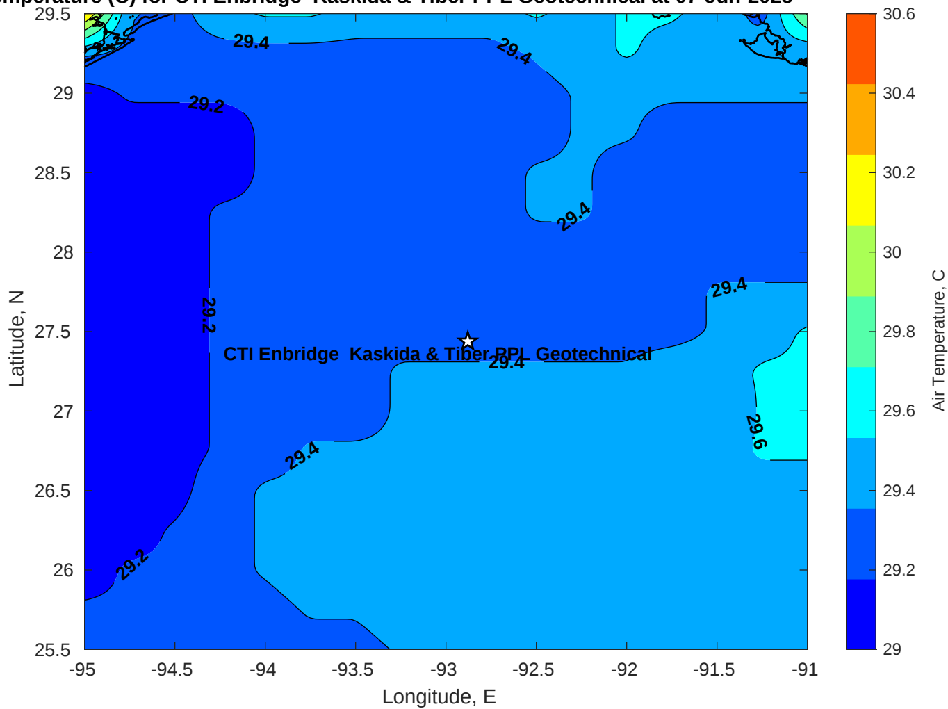
Air Temperature (C) for CTI Enbridge Kaskida & Tiber PPL Geotechnical at 07-Jun-2025
