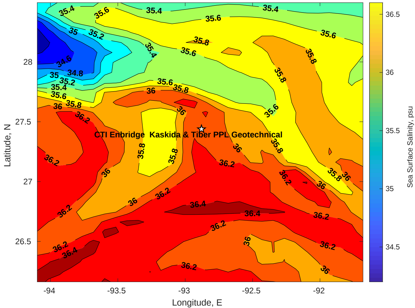
Surface Salinity for CTI Enbridge Kaskida & Tiber PPL Geotechnical at 06-Jun-2025 00:00:00
