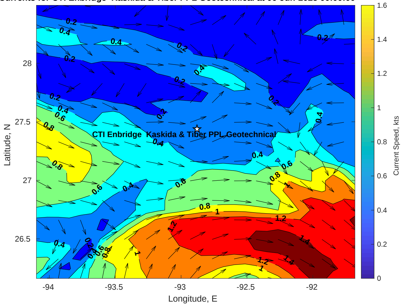
Surface Currents for CTI Enbridge Kaskida & Tiber PPL Geotechnical at 06-Jun-2025 00:00:00
