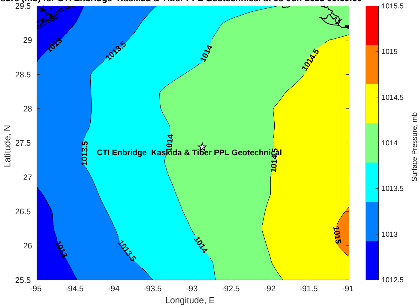
Surface Pressure (mb) for CTI Enbridge Kaskida & Tiber PPL Geotechnical at 08-Jun-2025 00:00:00
