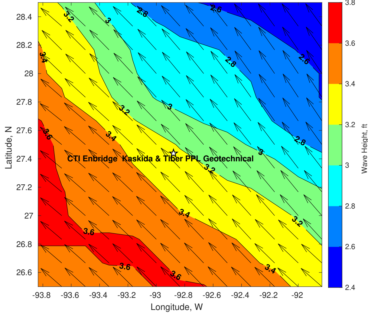
Wave Height (ft) for CTI Enbridge Kaskida & Tiber PPL Geotechnical at 07-Jun-2025 09:00:00
