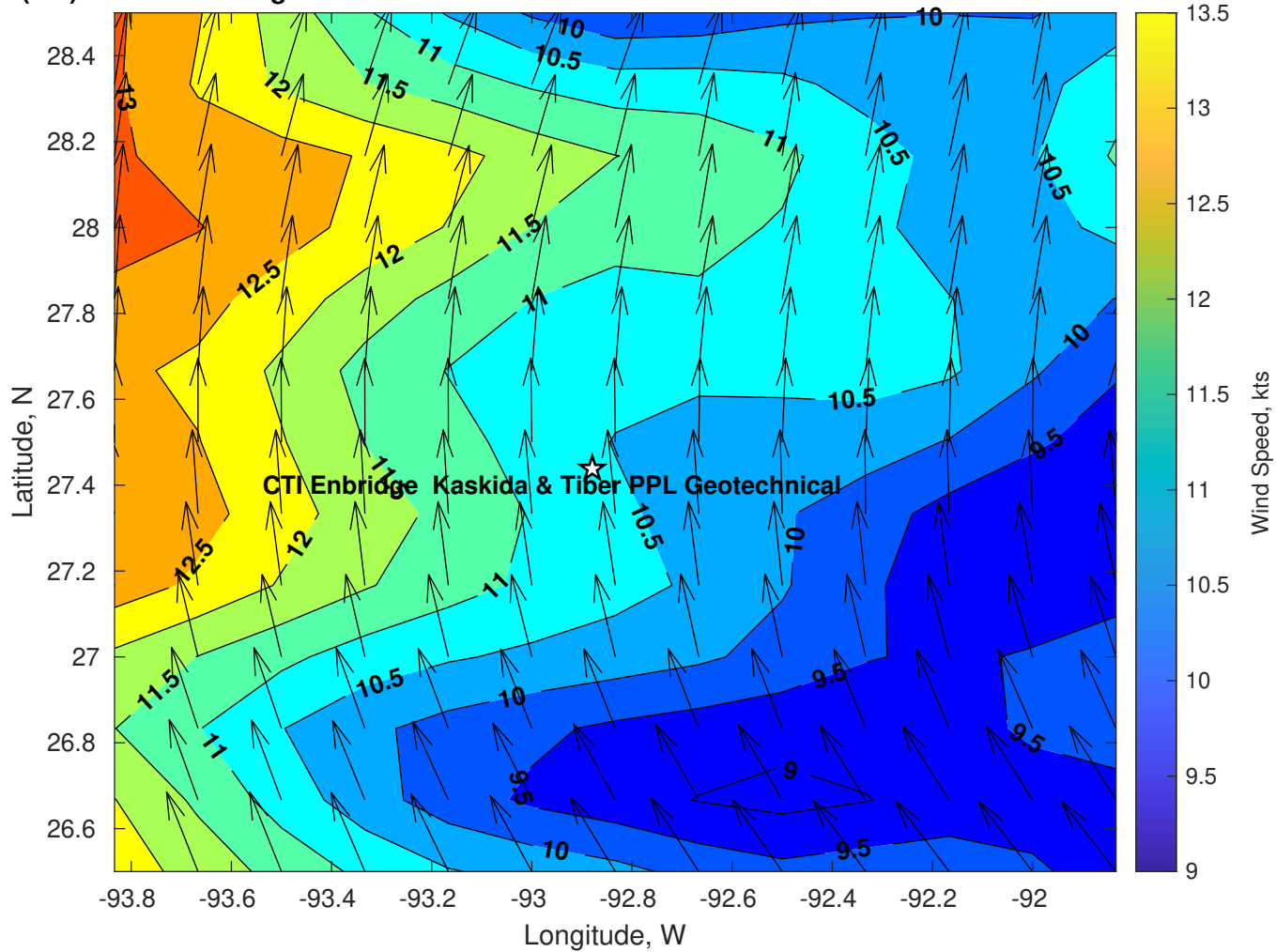
Winds (kts) for CTI Enbridge Kaskida & Tiber PPL Geotechnical at 07-Jun-2025 09:00:00
