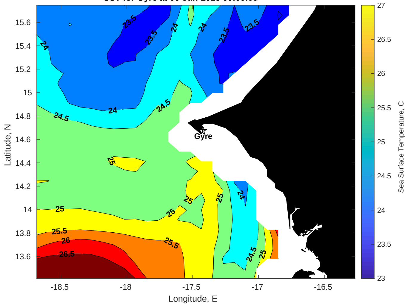
SST for Gyre at 06-Jun-2025 00:00:00
