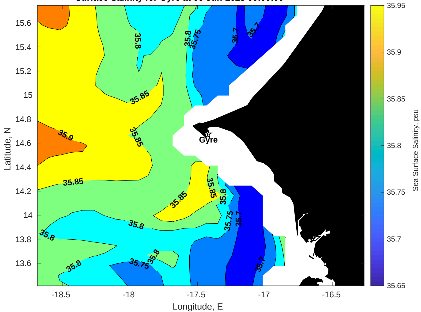
Surface Salinity for Gyre at 06-Jun-2025 00:00:00
