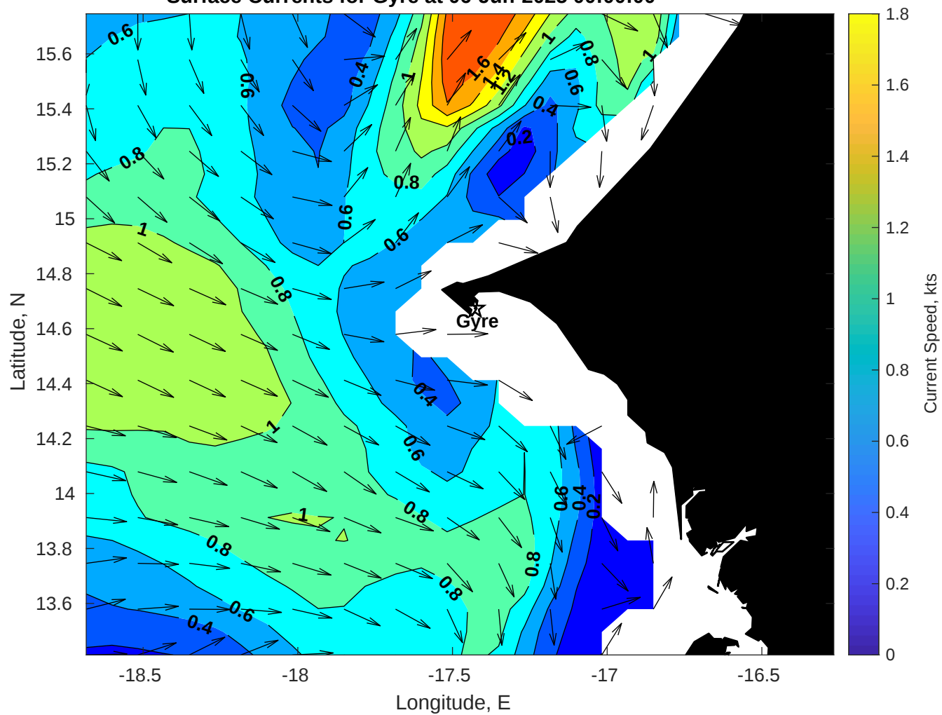
Surface Currents for Gyre at 06-Jun-2025 00:00:00
