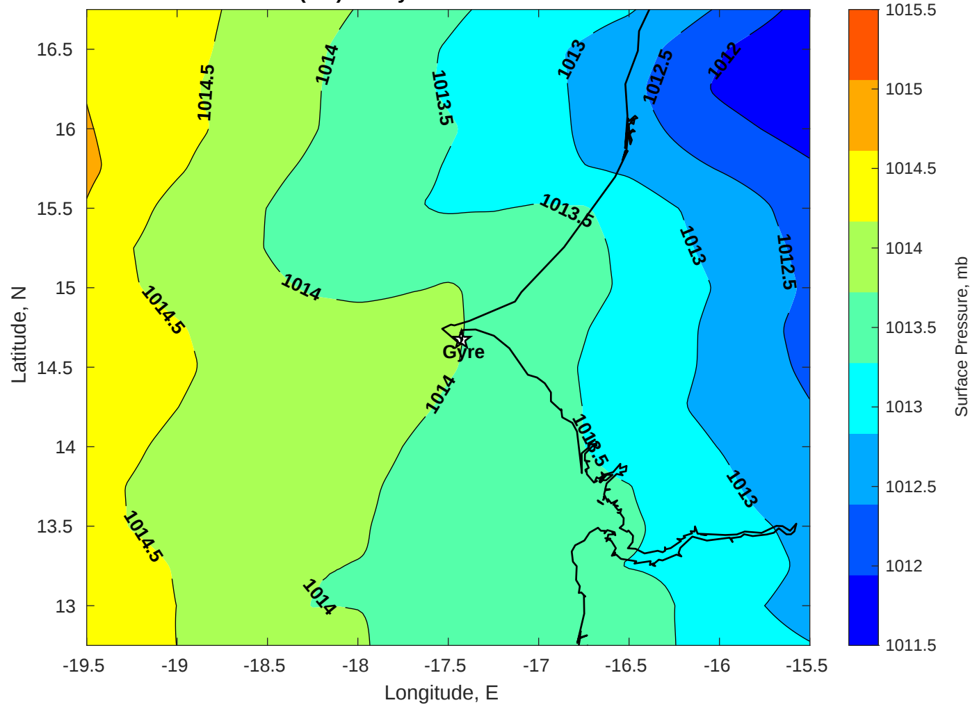
Surface Pressure (mb) for Gyre at 07-Jun-2025 00:00:00
