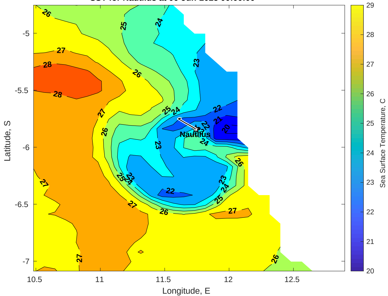
SST for Nautilus at 06-Jun-2025 00:00:00
