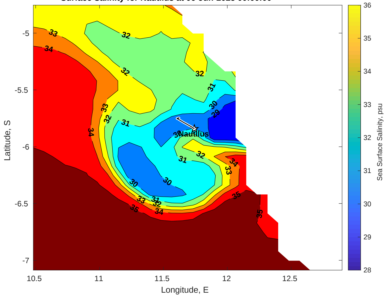
Surface Salinity for Nautilus at 06-Jun-2025 00:00:00
