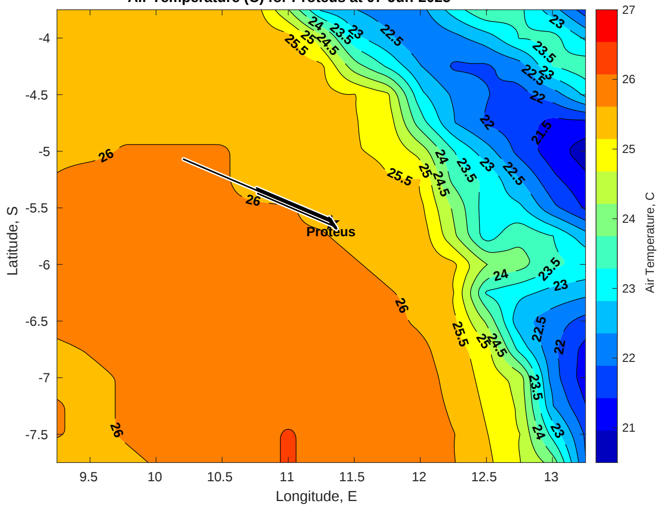
Air Temperature (C) for Proteus at 07-Jun-2025
