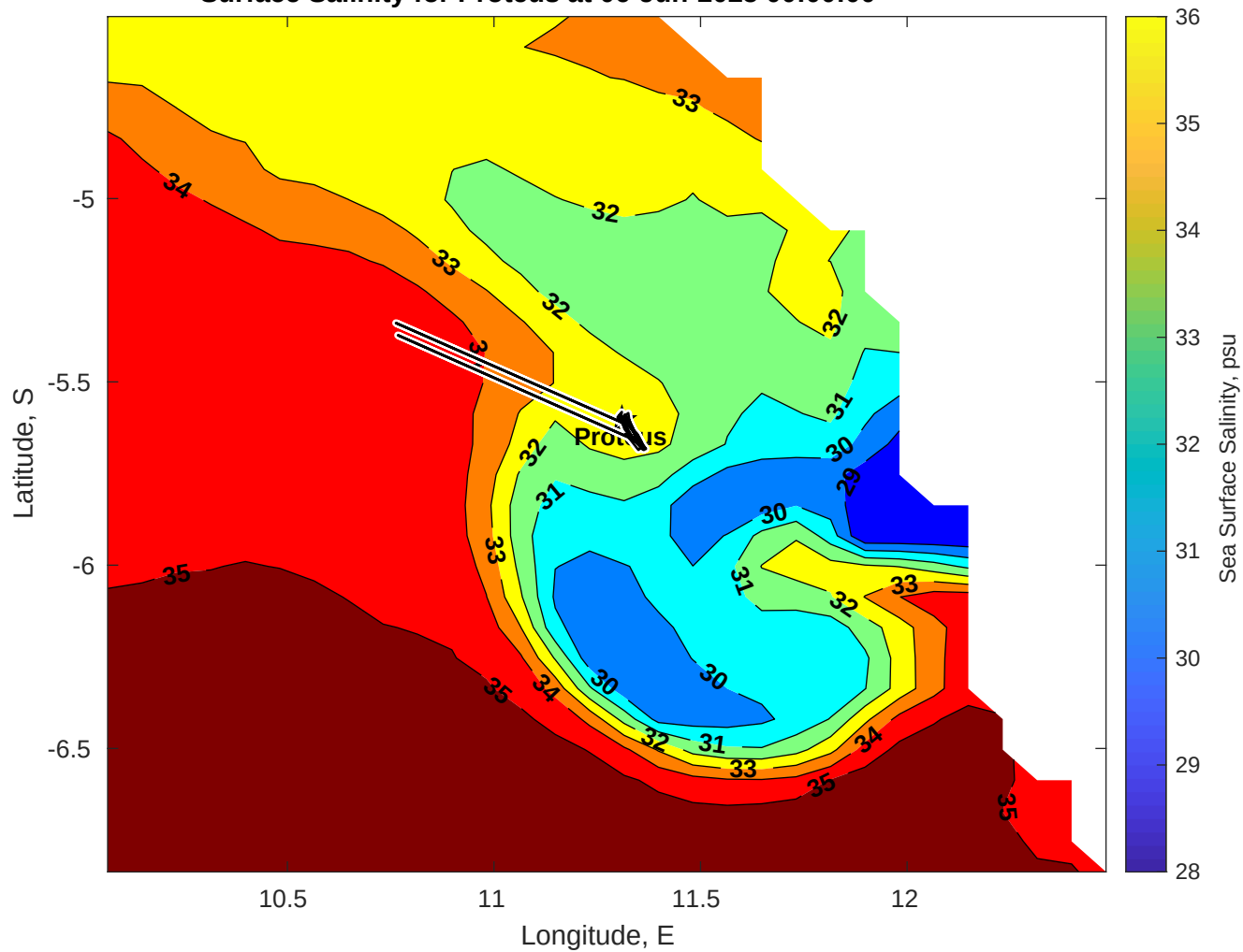
Surface Salinity for Proteus at 06-Jun-2025 00:00:00
