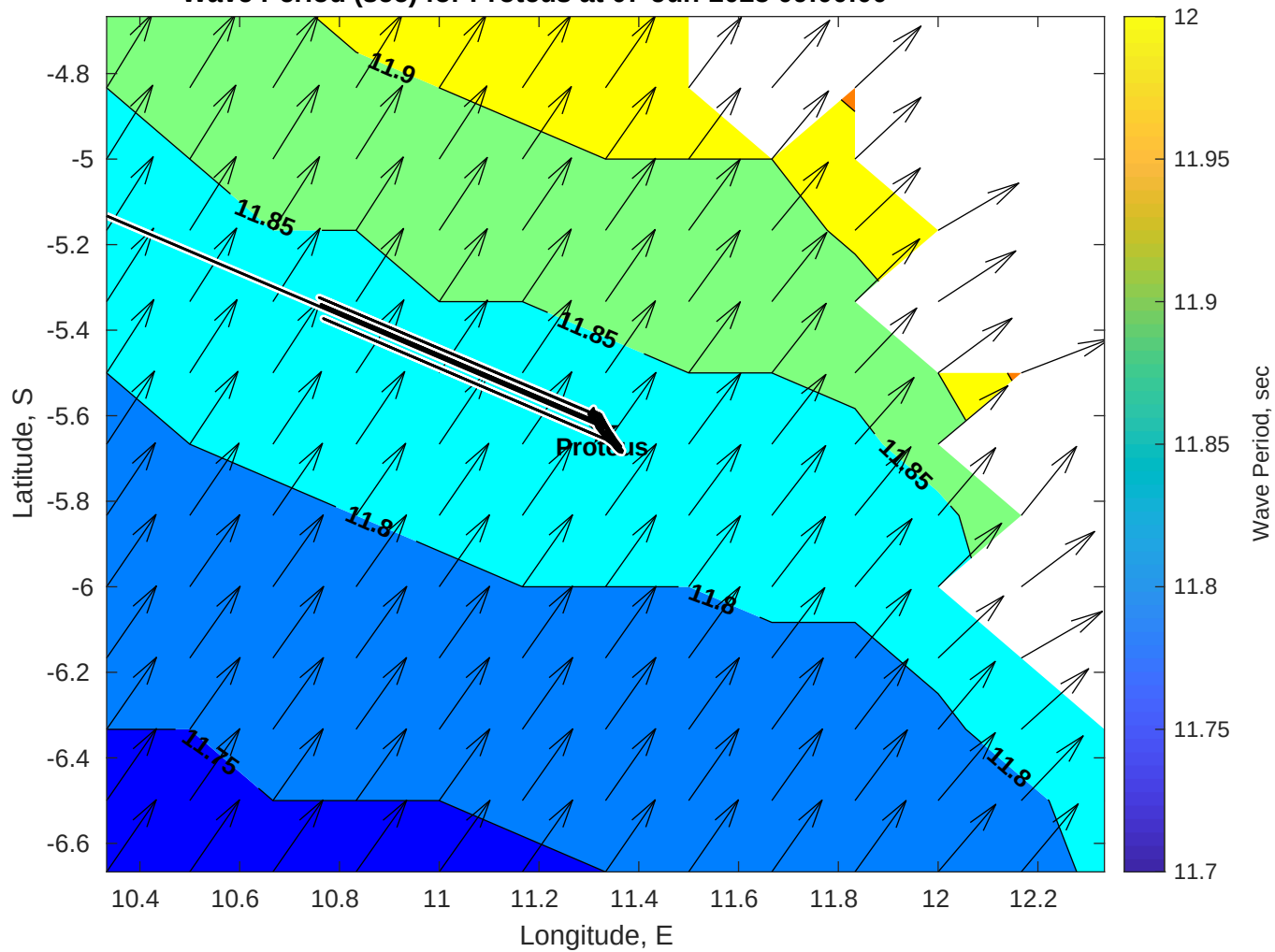
Wave Period (sec) for Proteus at 07-Jun-2025 09:00:00
