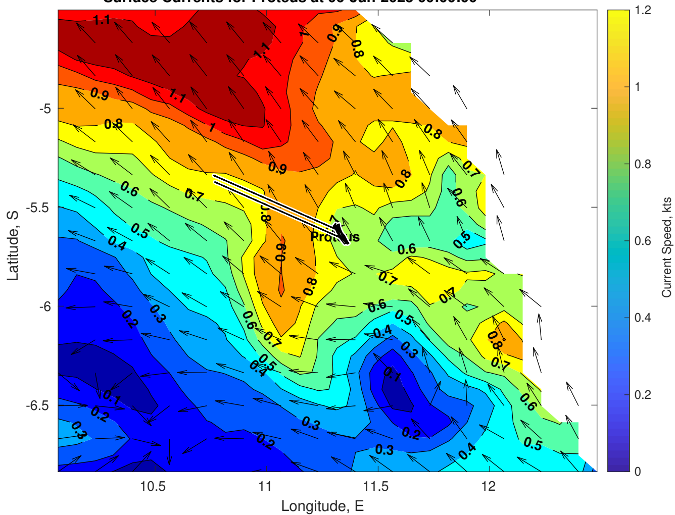
Surface Currents for Proteus at 06-Jun-2025 00:00:00
