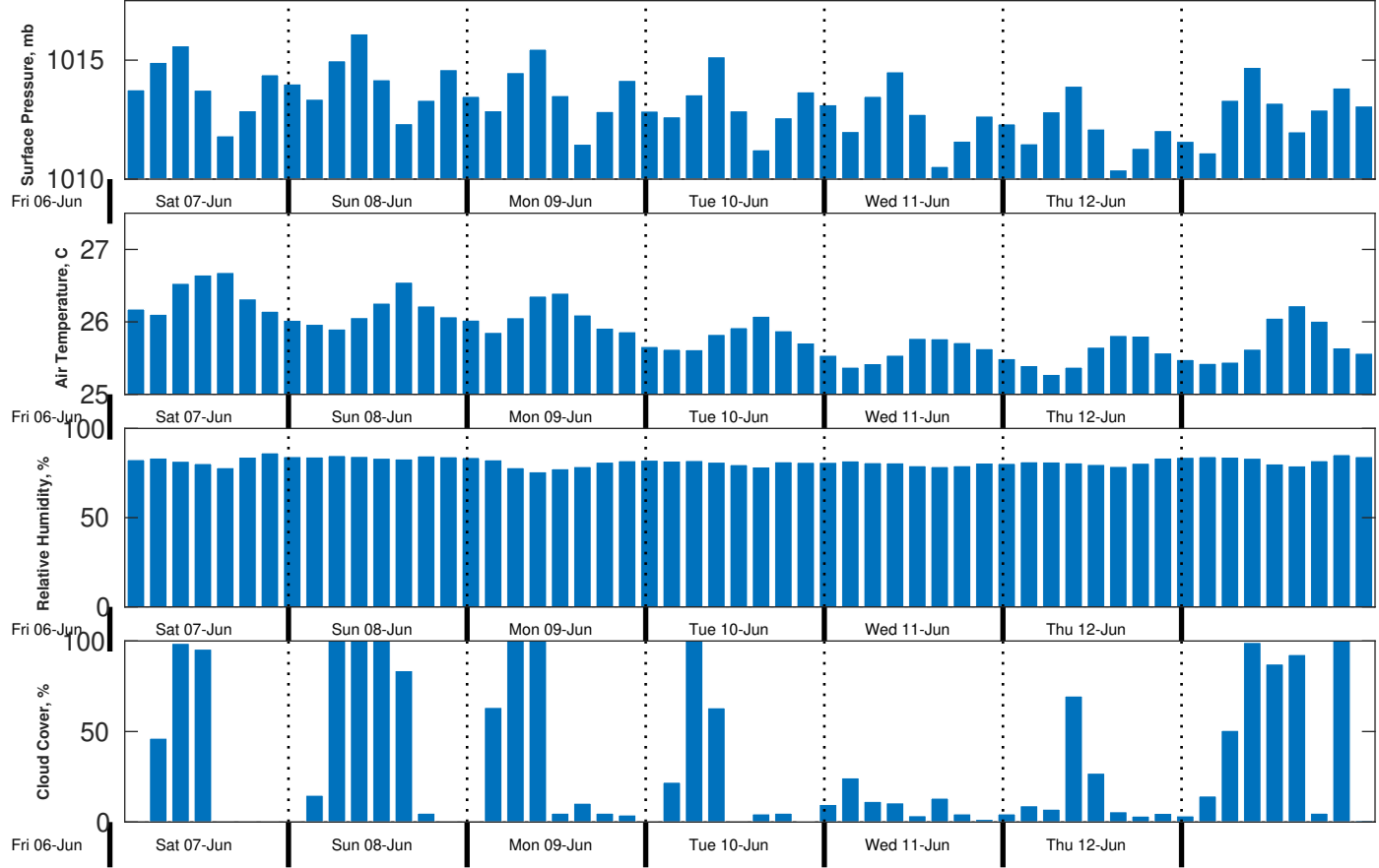
Met Forecast for Proteus from 07-Jun-2025 00:00:00 to 14-Jun-2025 00:00:00
