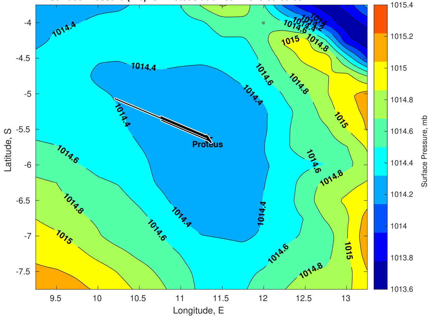
Surface Pressure (mb) for Proteus at 07-Jun-2025 00:00:00
