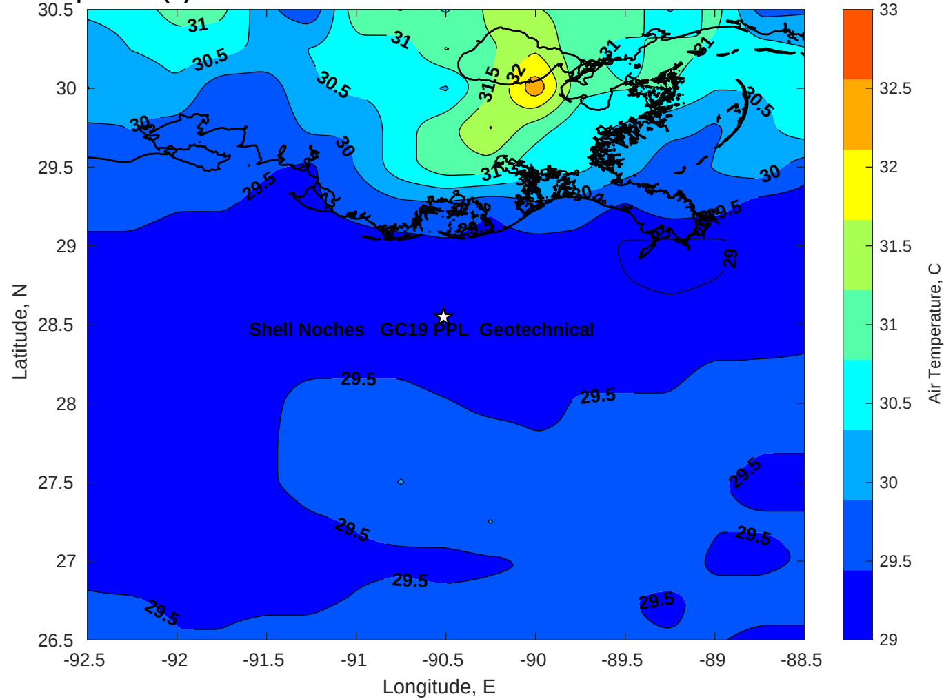
Air Temperature (C) for Shell Noches GC19 PPL Geotechnical at 07-Jun-2025
