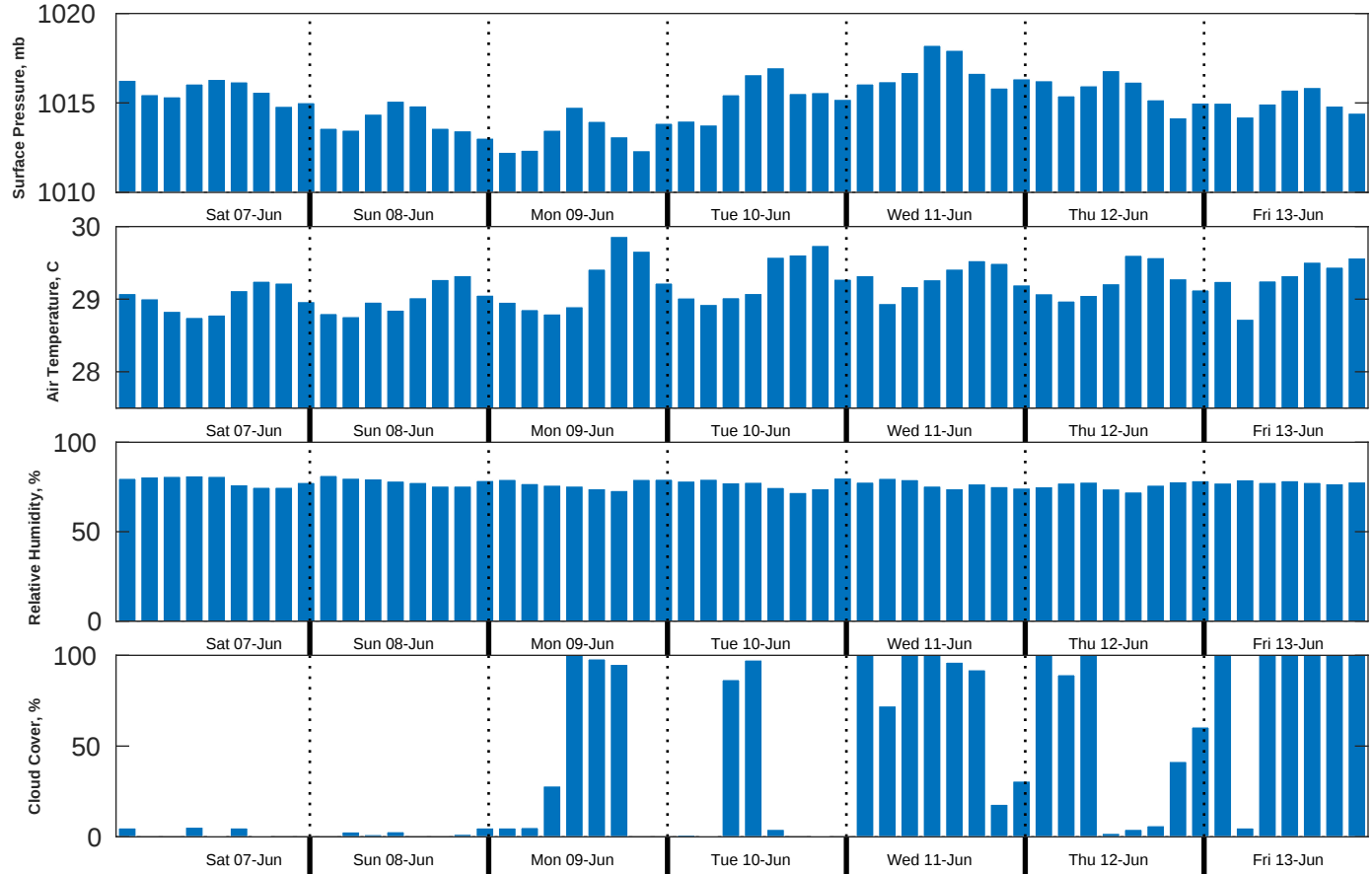
Met Forecast for Shell Noches GC19 PPL Geotechnical from 07-Jun-2025 00:00:00 to 14-Jun-2025 00:00:00
