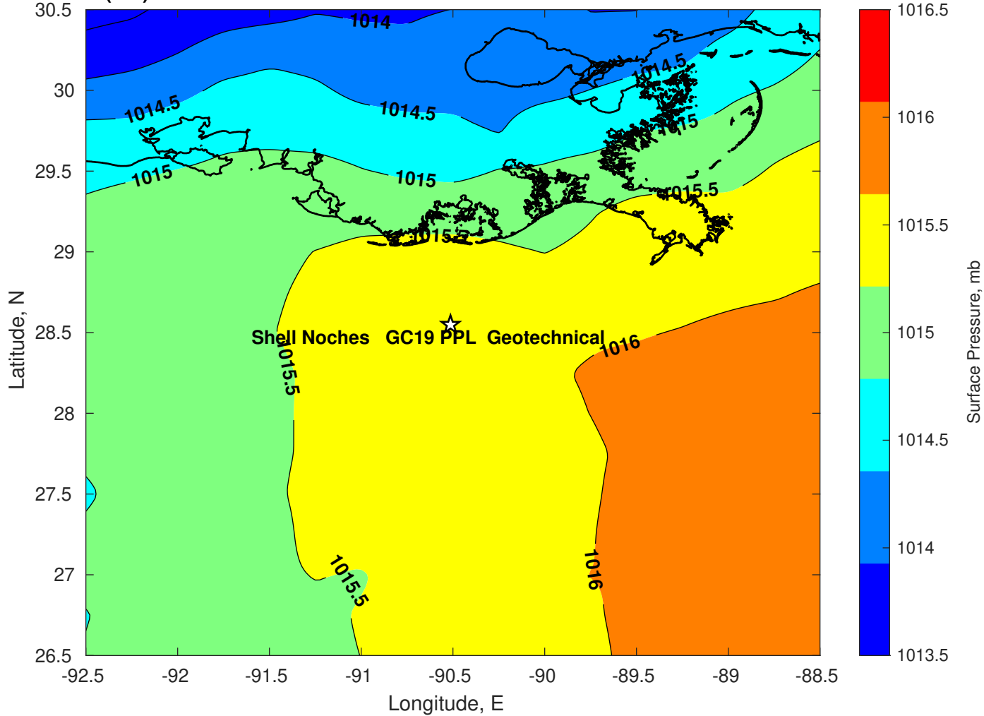
Surface Pressure (mb) for Shell Noches GC19 PPL Geotechnical at 07-Jun-2025 00:00:00
