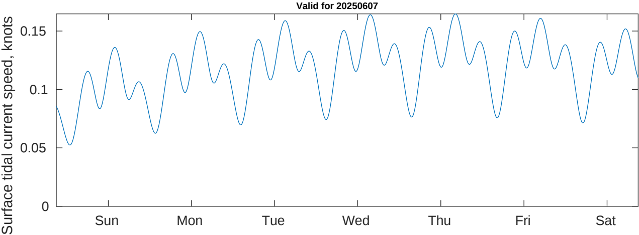
Tidal Currents and Heights for Shell Noches GC19 PPL Geotechnical at 20250607
