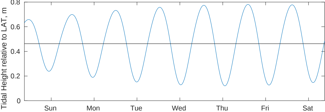
Tidal Currents and Heights for Shell Noches GC19 PPL Geotechnical at 20250607
