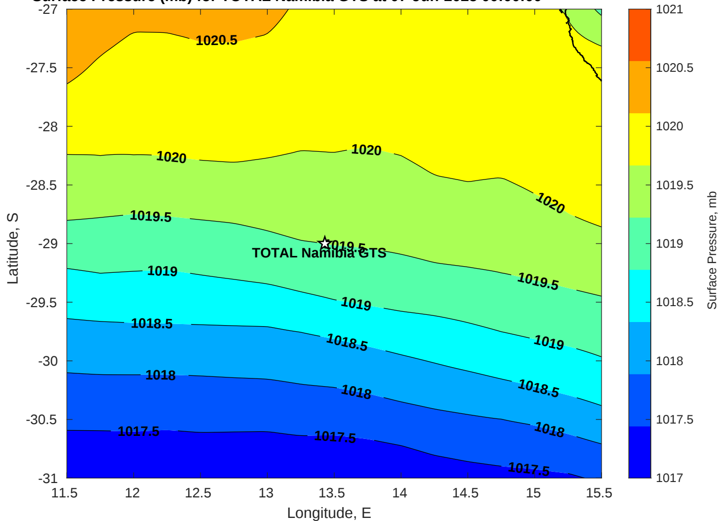
Surface Pressure (mb) for TOTAL Namibia GTS at 07-Jun-2025 00:00:00
