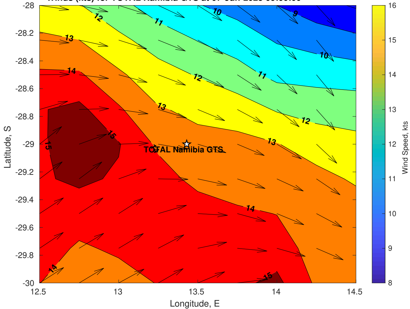
Winds (kts) for TOTAL Namibia GTS at 07-Jun-2025 09:00:00
