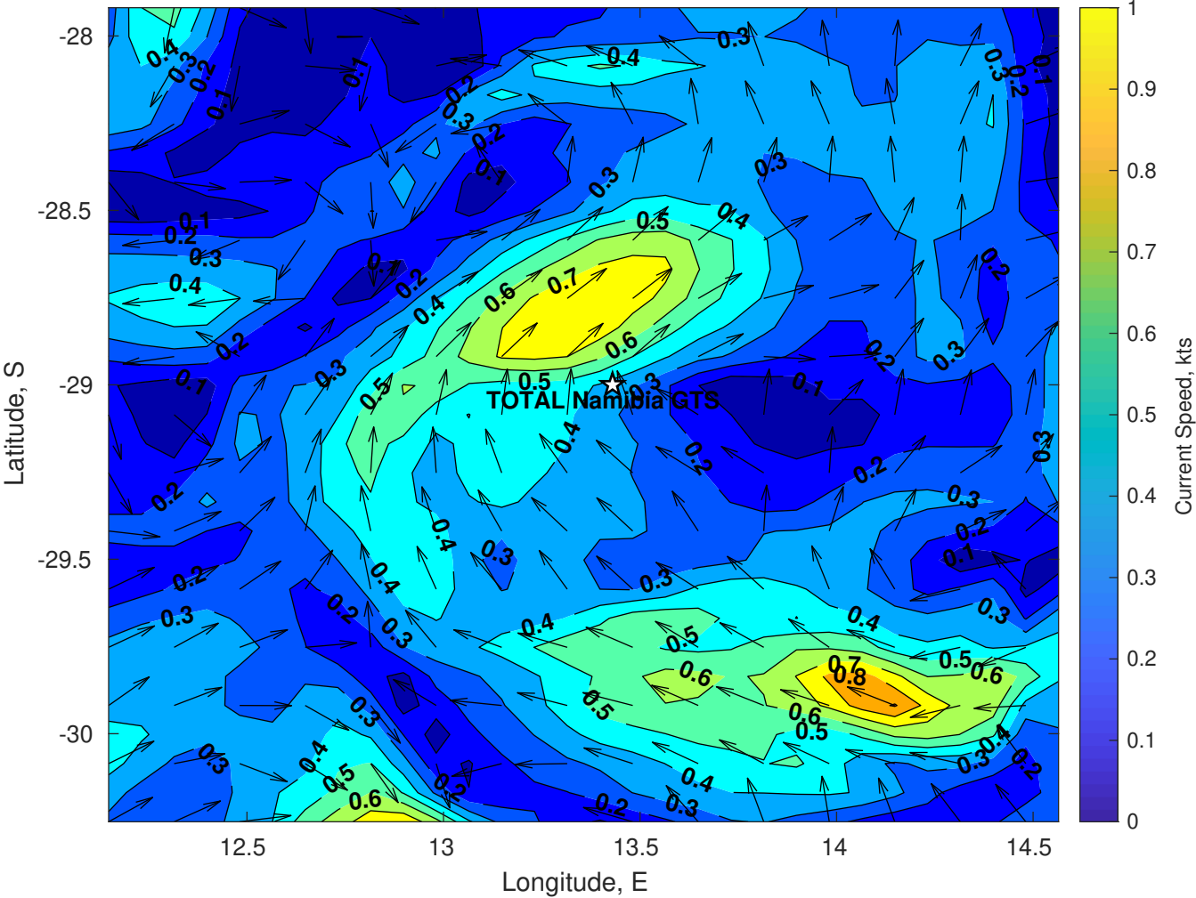
Surface Currents for TOTAL Namibia GTS at 06-Jun-2025 00:00:00
