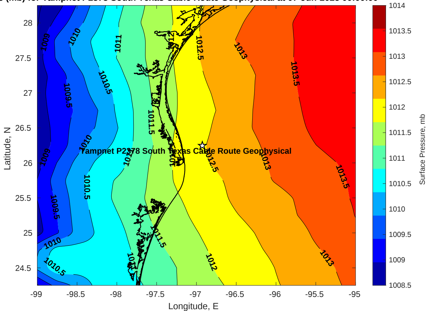
Pressure (mb) for Tampnet P2378 South Texas Cable Route Geophysical at 07-Jun-2025 00:00:00
