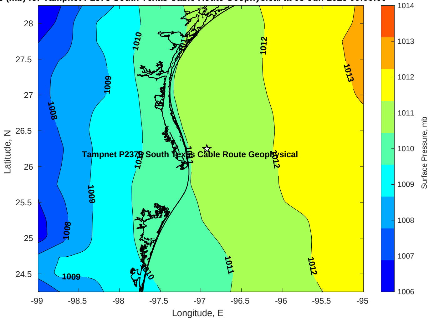
Pressure (mb) for Tampnet P2378 South Texas Cable Route Geophysical at 08-Jun-2025 00:00:00
