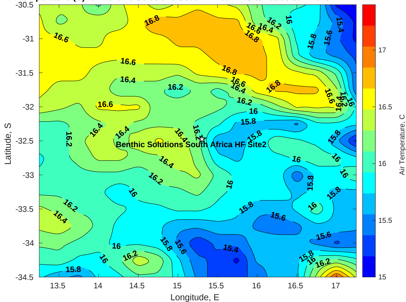
Air Temperature (C) for Benthic Solutions South Africa HF Site2 at 08-Jun-2025
