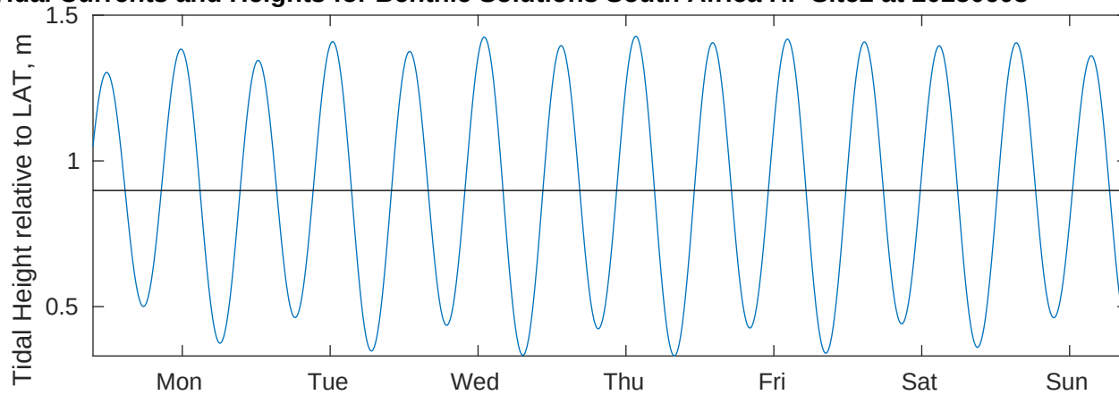
Tidal Currents and Heights for Benthic Solutions South Africa HF Site2 at 20250608
