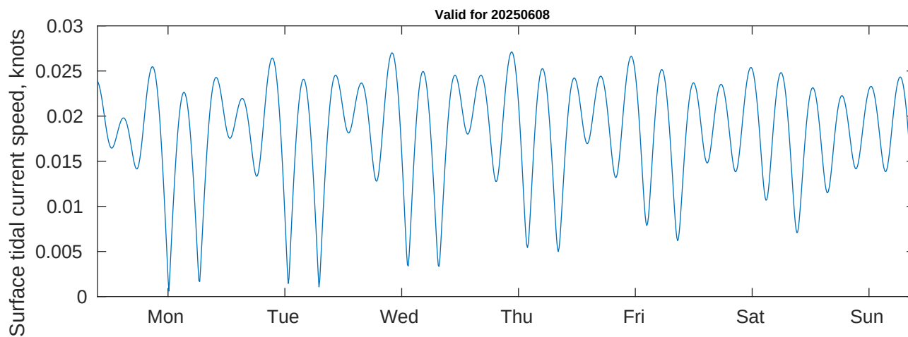
Tidal Currents and Heights for Benthic Solutions South Africa HF Site2 at 20250608
