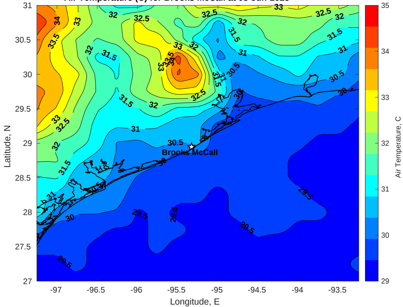
Air Temperature (C) for Brooks McCall at 08-Jun-2025
