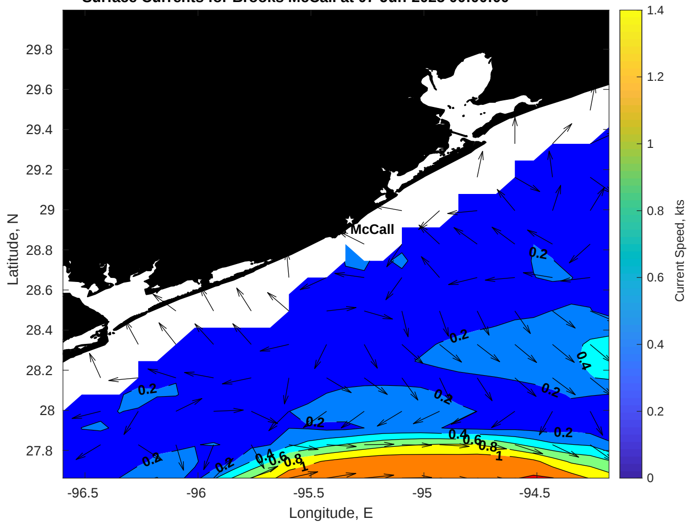
Surface Currents for Brooks McCall at 07-Jun-2025 00:00:00
