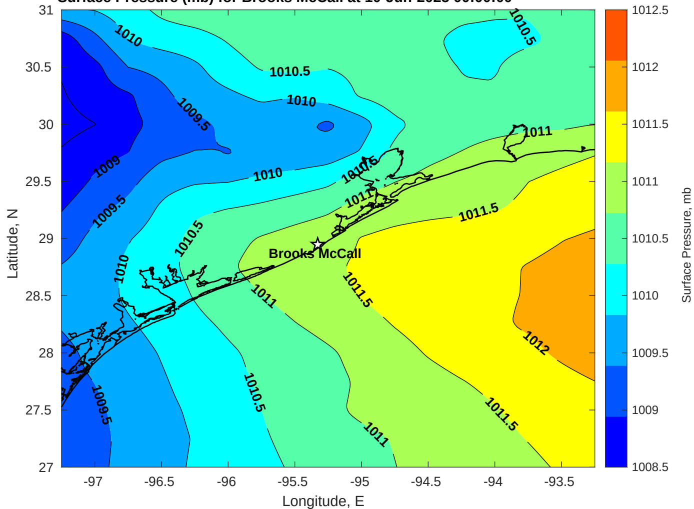
Surface Pressure (mb) for Brooks McCall at 10-Jun-2025 00:00:00
