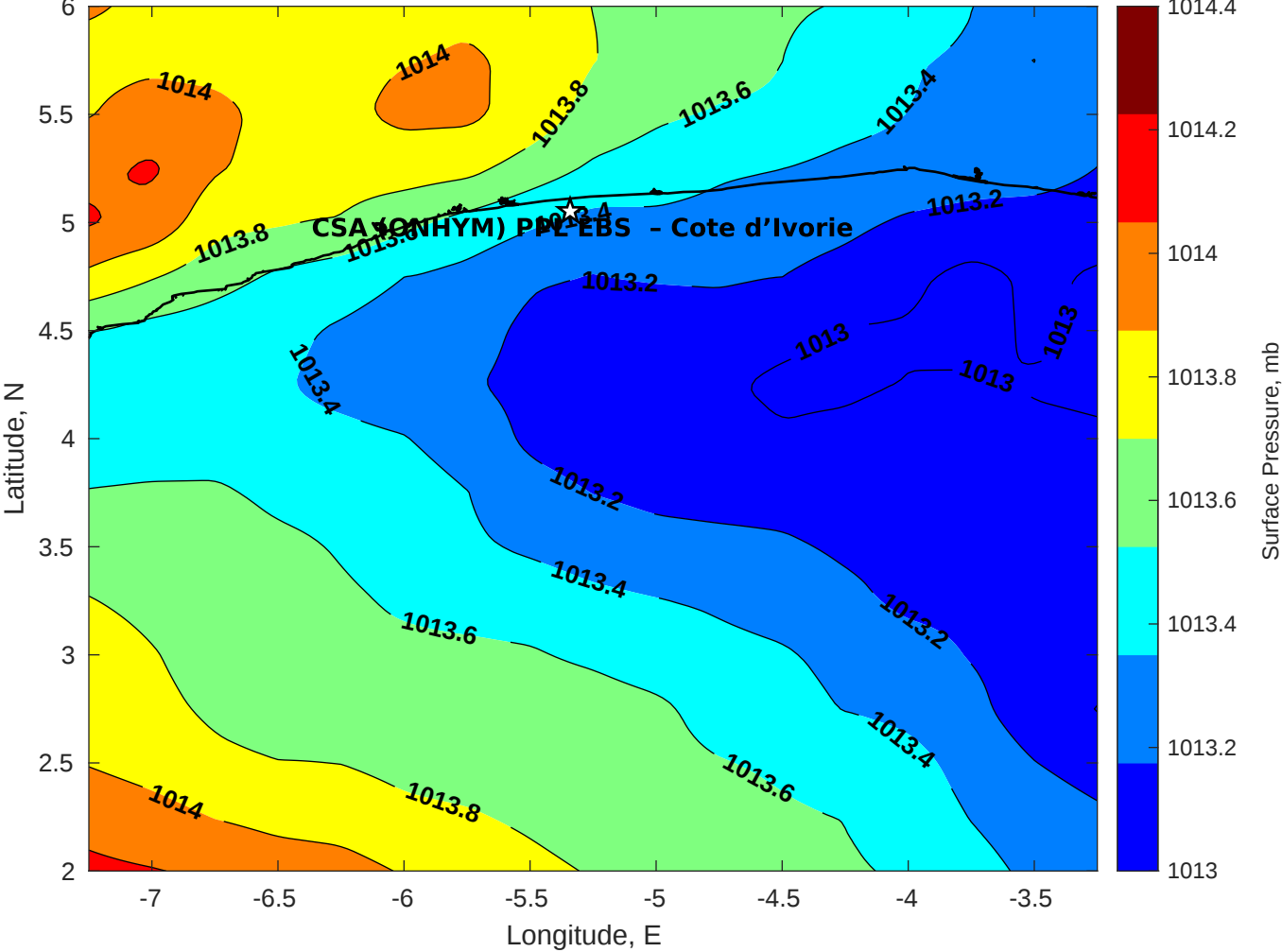
Surface Pressure (mb) for CSA (ONHYM) PPL EBS - Cote d'Ivoire at 10-Jun-2025 00:00:00
