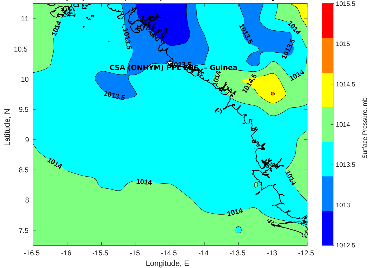
Surface Pressure (mb) for CSA (ONHYM) PPL EBS - Guinea at 10-Jun-2025 00:00:00
