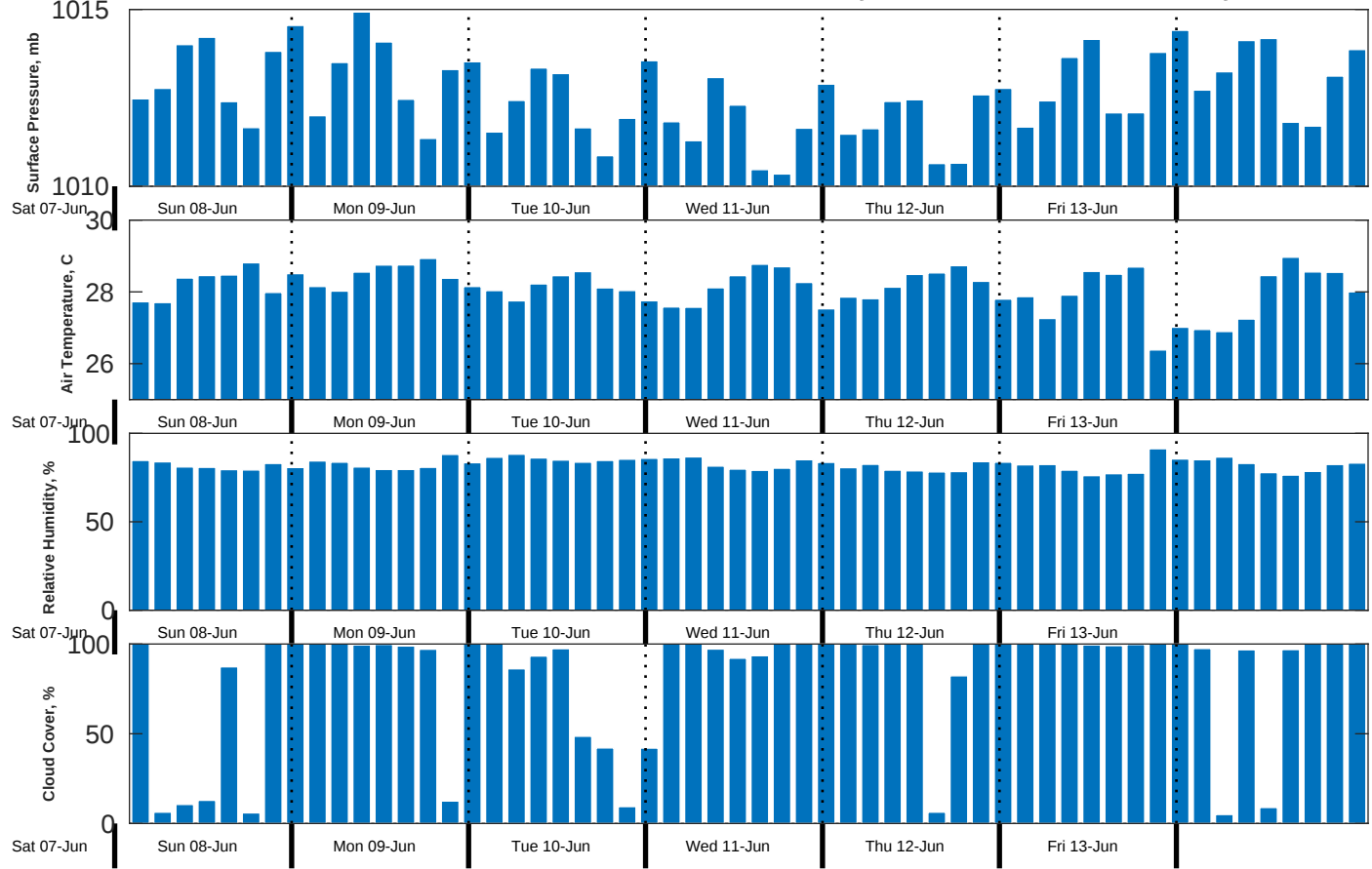
Met Forecast for CSA (ONHYM) PPL EBS - Guinea from 08-Jun-2025 00:00:00 to 15-Jun-2025 00:00:00
