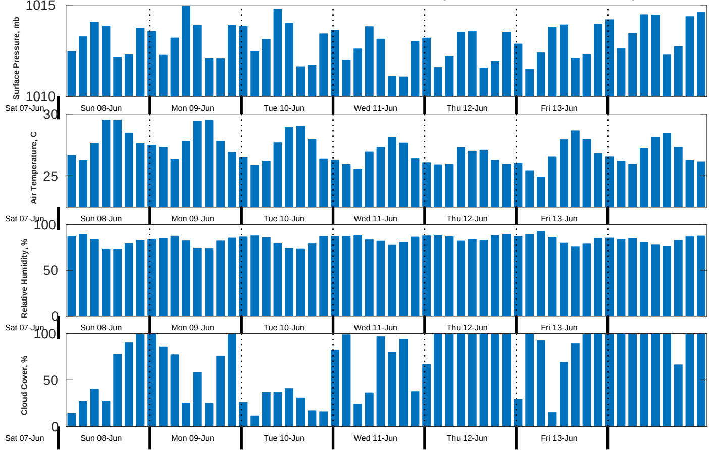
Met Forecast for CSA (ONHYM) PPL EBS - Liberia from 08-Jun-2025 00:00:00 to 15-Jun-2025 00:00:00
